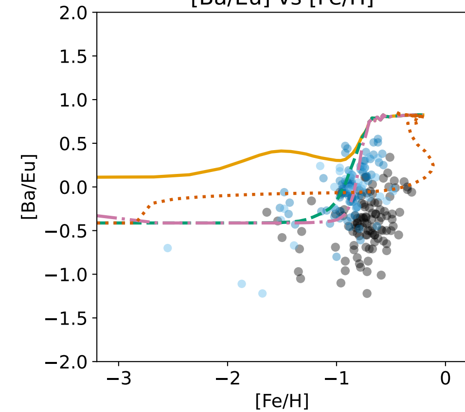
[Ba/Eu] vs [Fe/H]
