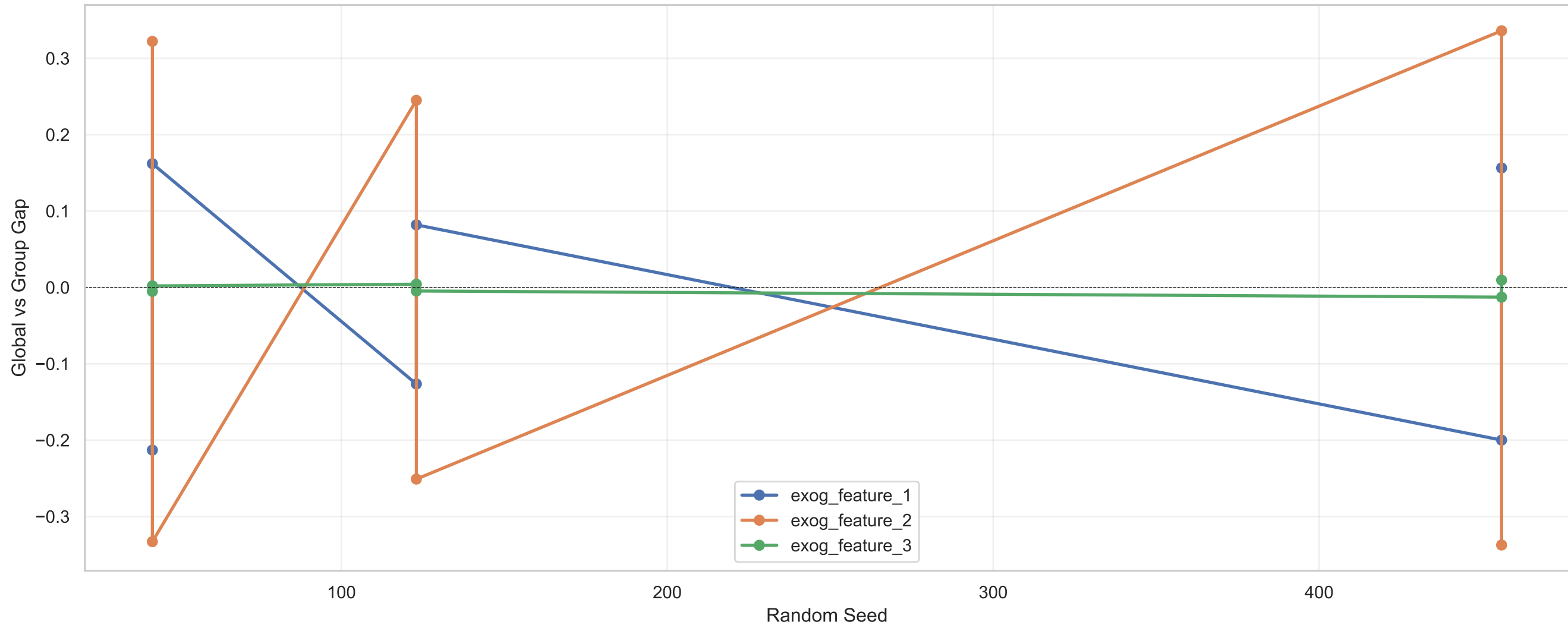
Feature Importance Gap Stability Across Seeds
