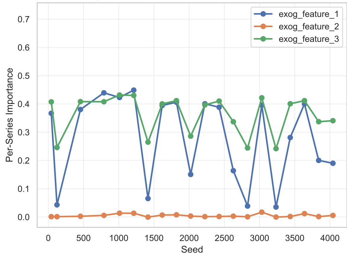
group_a: Per-Series Importance Across Seeds
