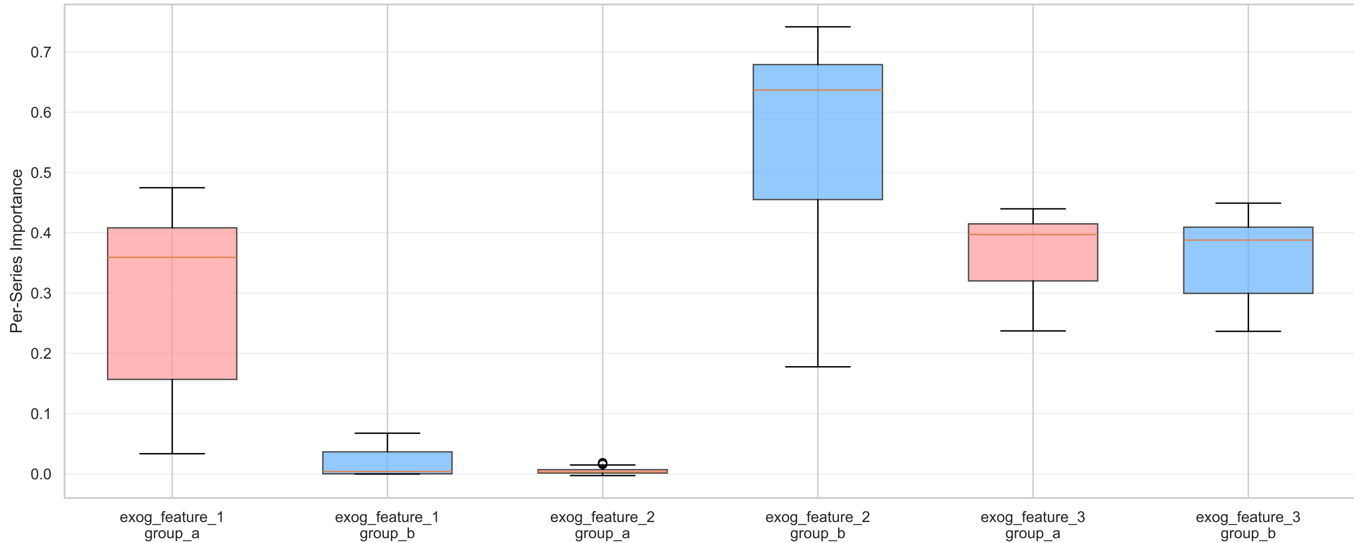
Box Plot: Per-Series Feature Importance Distribution by Group
