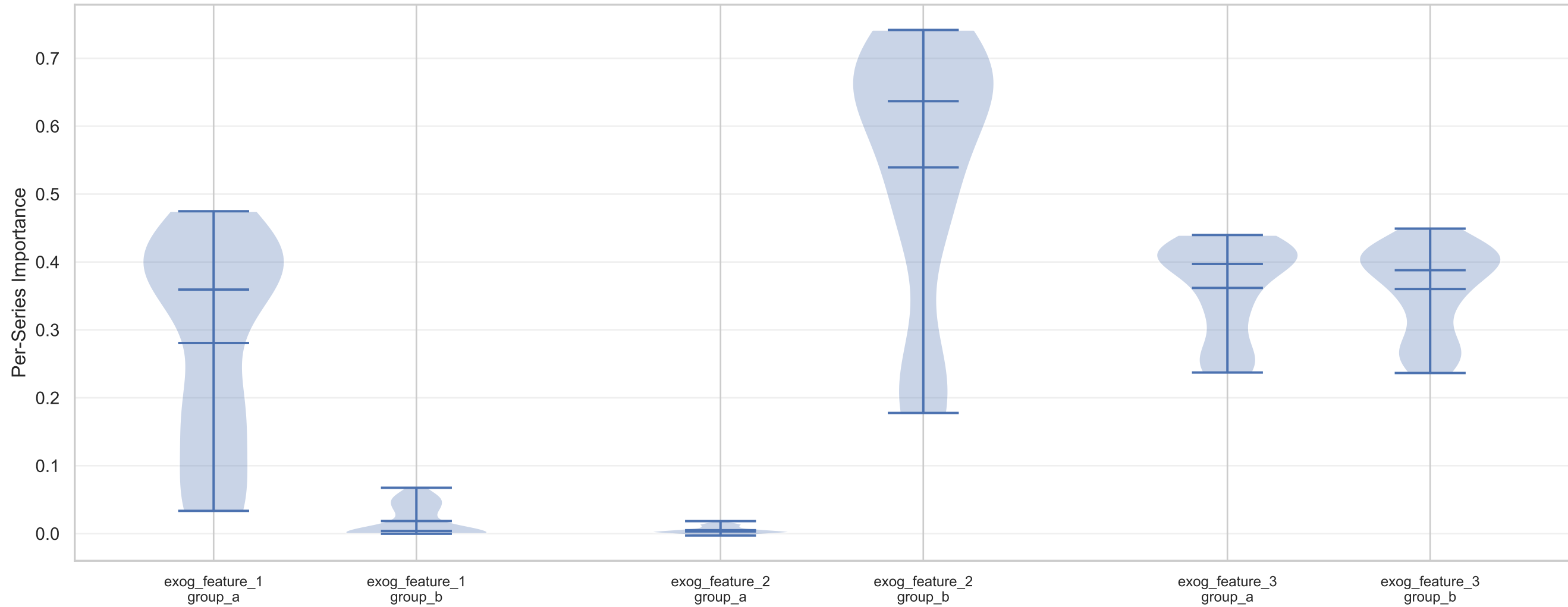
Distribution of Per-Series Feature Importance (Across all series and seeds)
