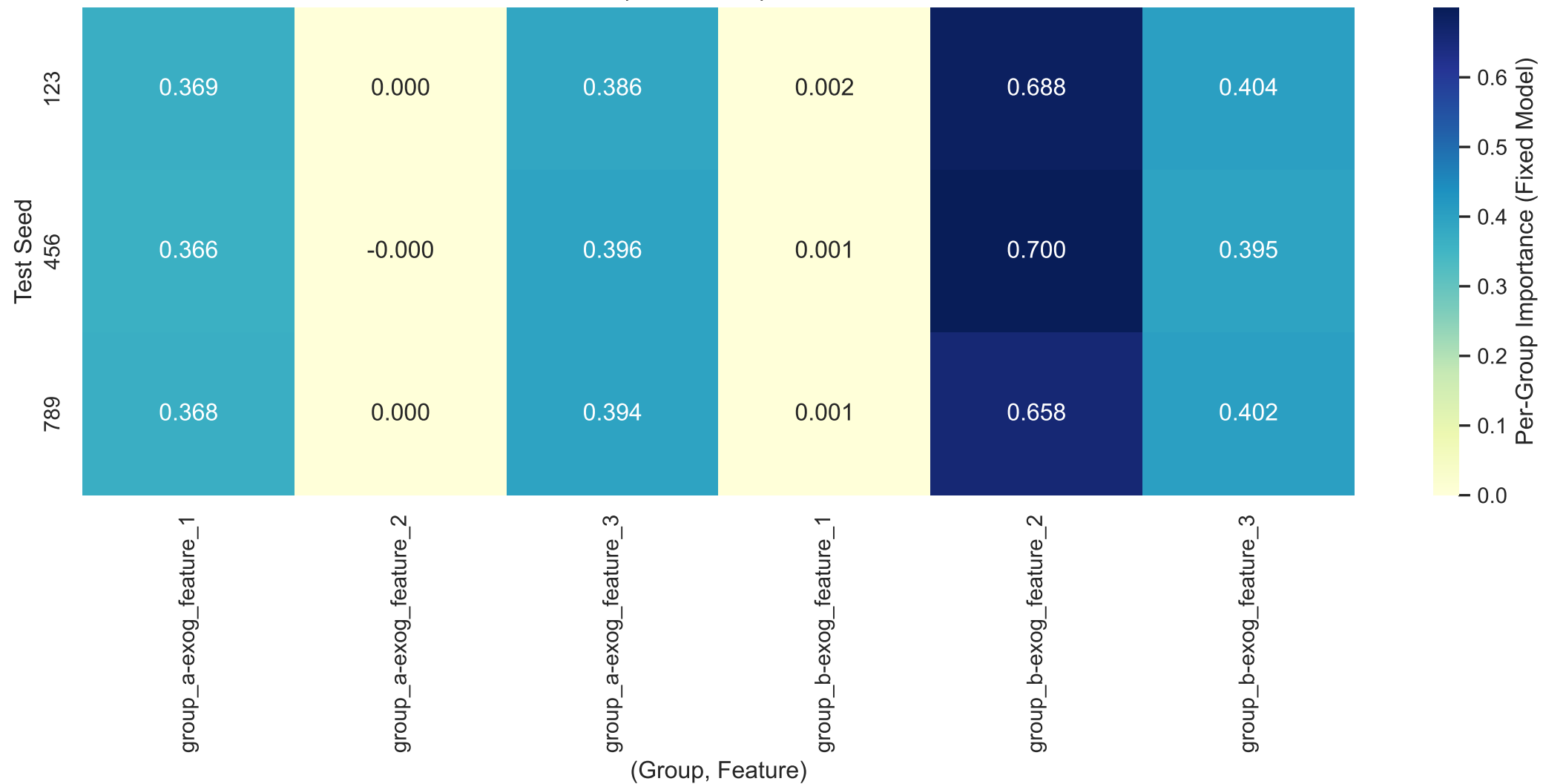
Fixed Model: Per-Group Feature Importance Across Test Seeds
