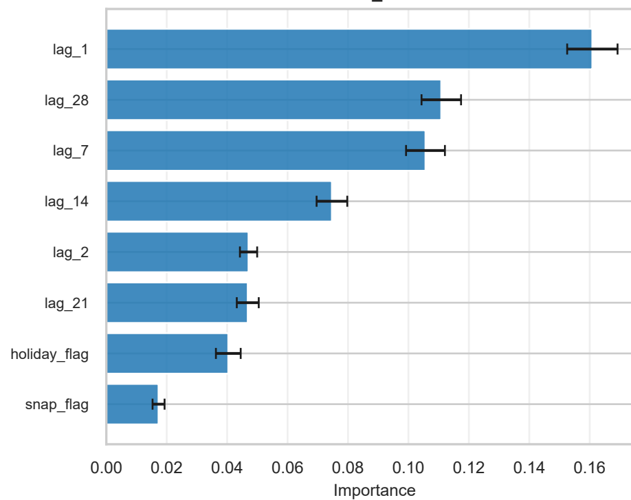
Series: WI_HOBBIES
