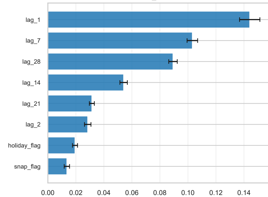
Series: TX_HOUSEHOLD
