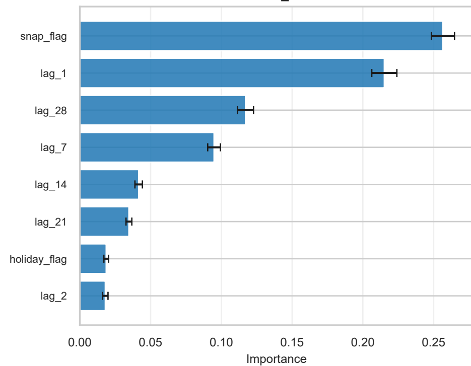
Series: WI_FOODS
