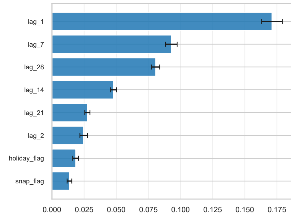
Series: WI_HOUSEHOLD
