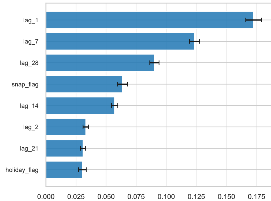
Series: TX_FOODS
