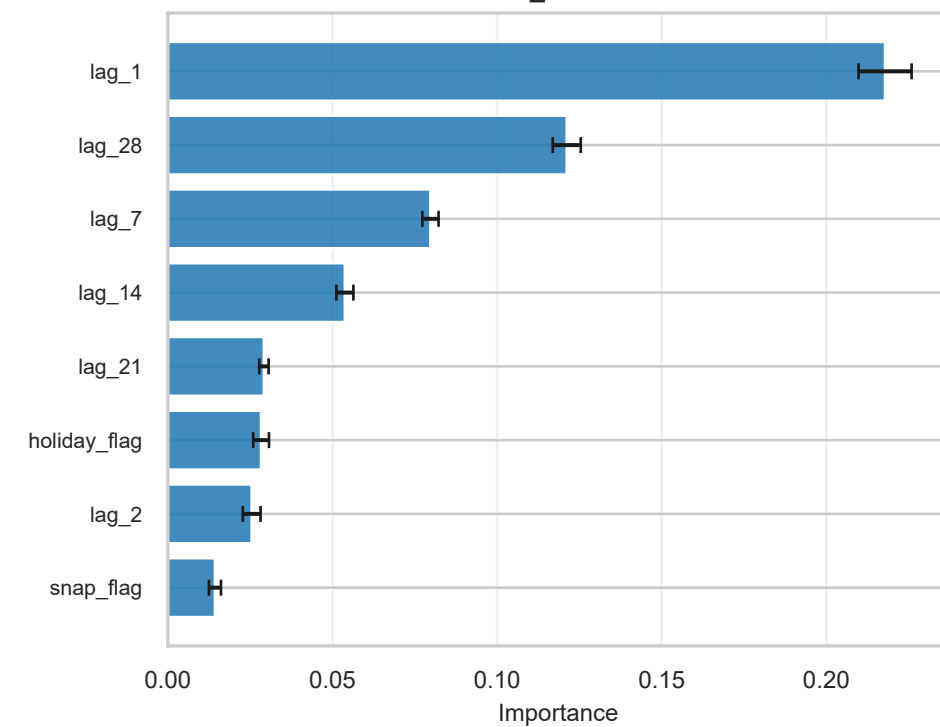
Series: WI_HOUSEHOLD
