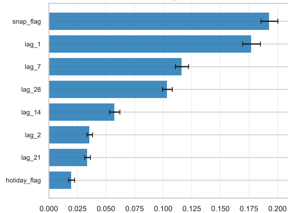
Series: WI_FOODS
