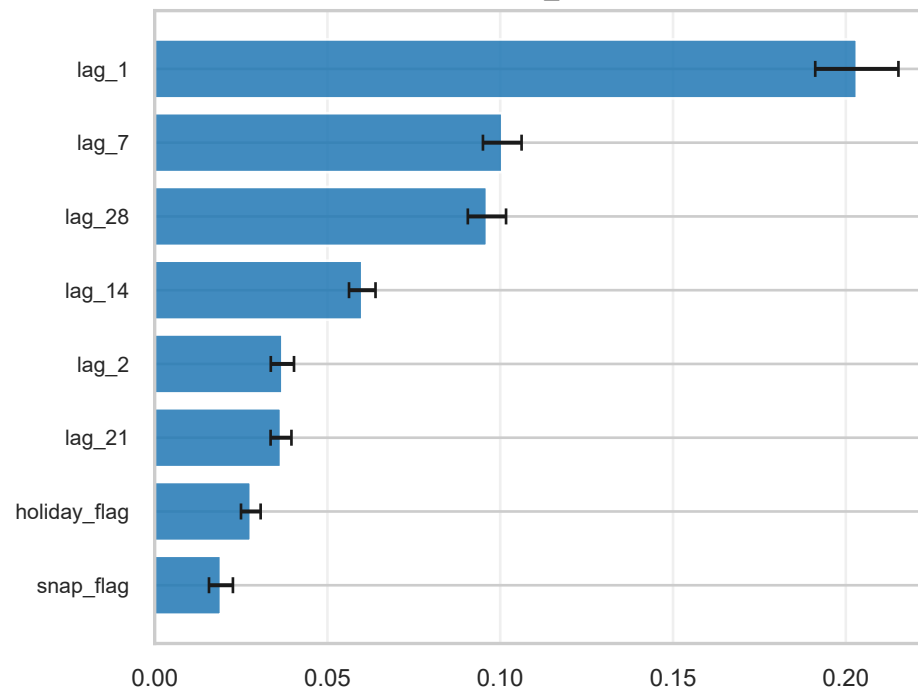
Series: TX_HOBBIES
