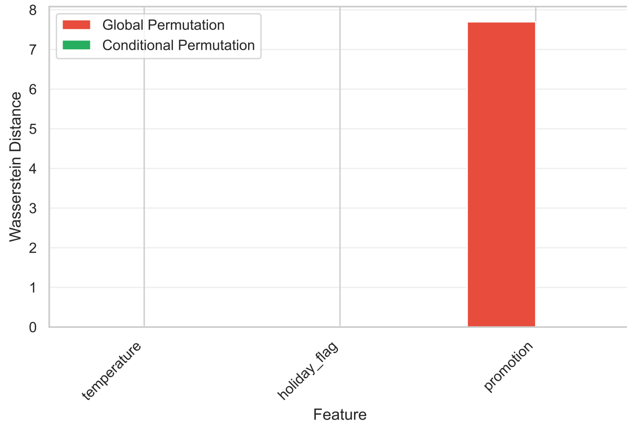
Distribution Shift: Wasserstein Distance
