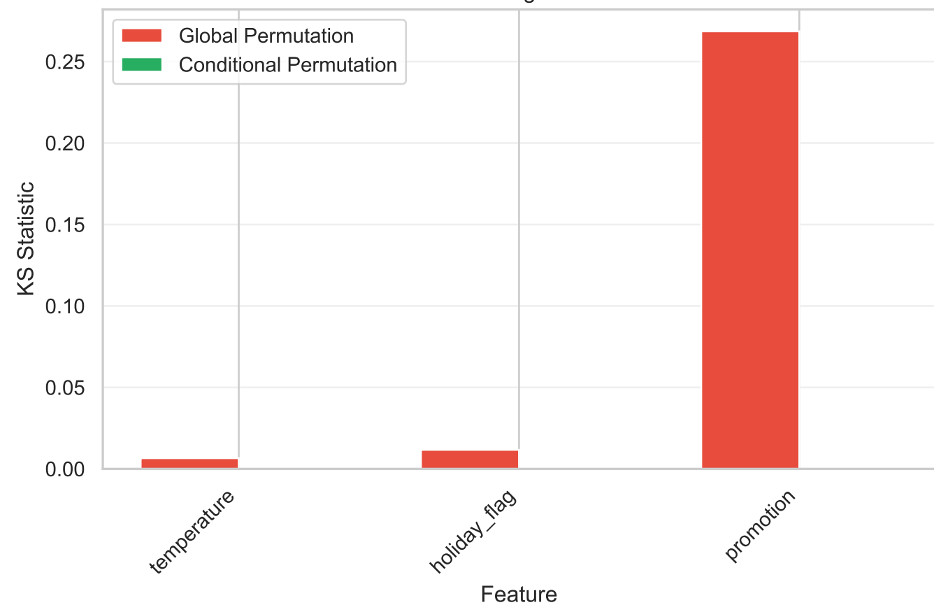
Distribution Shift: Kolmogorov-Smirnov Statistic
