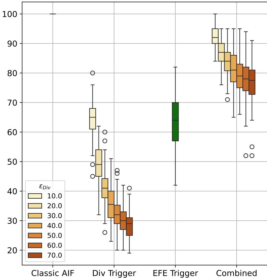
Number of Planning Phases
