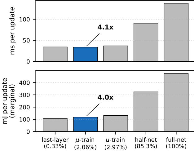
Fig. 2. Per-update wall-time (top) and marginal energy above the 2.77 W idle baseline (bottom) vs. trainable-parameter fraction. The \mu -training point at 2.06% (blue) lies on the flat regime; cost climbs sharply above \sim 3\% as further convolutional layers enter the backward pass. Raspberry Pi 5, 4 threads, batch 32, seq. length 250, FP32, SGD; peripheral draw excluded from PMIC totals (see body text).
