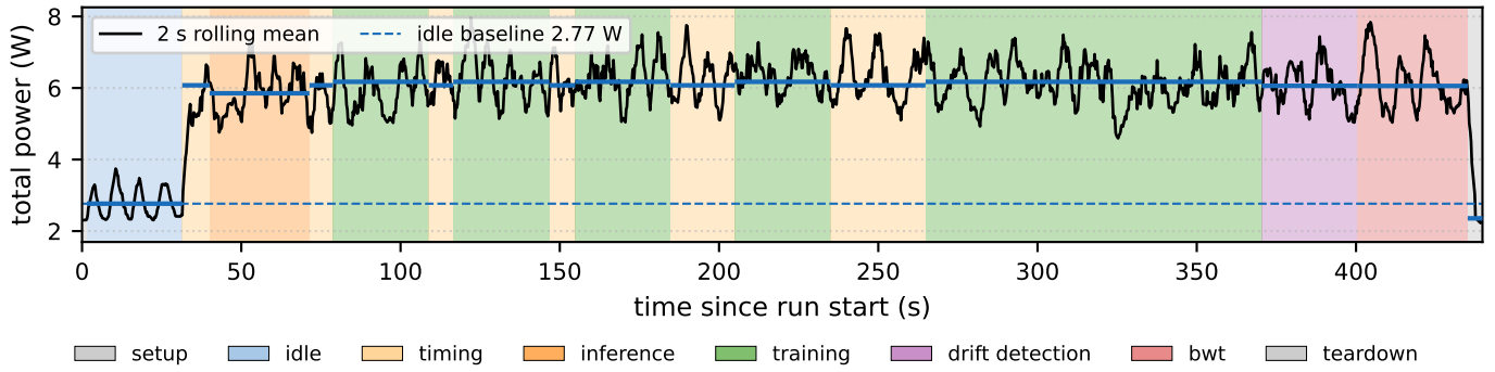
Fig. 3. PMIC power telemetry over the 440s pilot run. Colour bands: active pipeline phase; grey trace: raw 5 Hz samples (14 rails summed via vcgencmd pmic_read_adc ); black trace: 2s rolling mean; dashed line: 2.77 W idle reference. The five training plateaus correspond to the trainable-fraction sweep; the two rightmost ( half-net , full-net ) show visibly longer per-update settle times.
