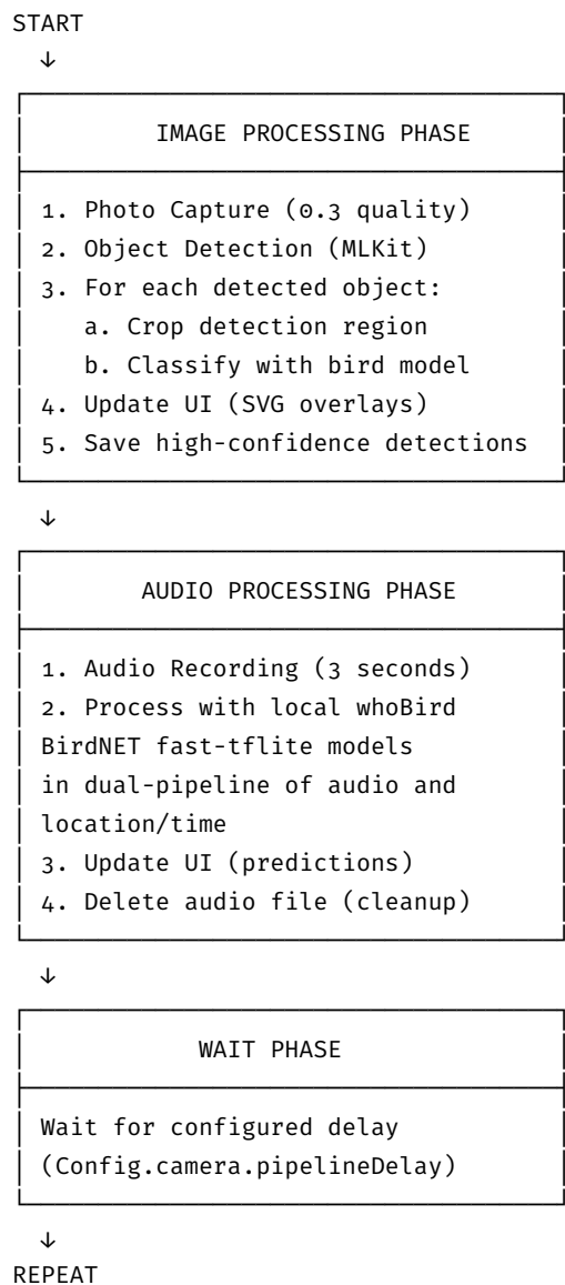
Abb. 4.2.: Unified ML Pipeline Processing Flow
