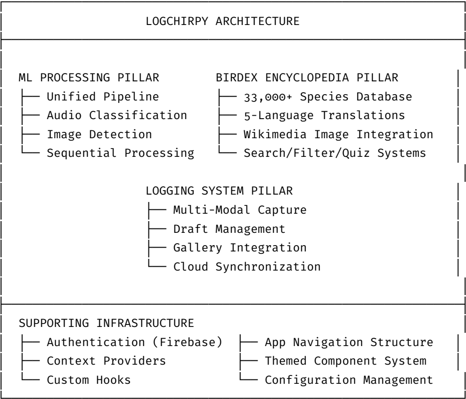
Abb. 4.1.: LogChirpy’s Three-Pillar Architecture
