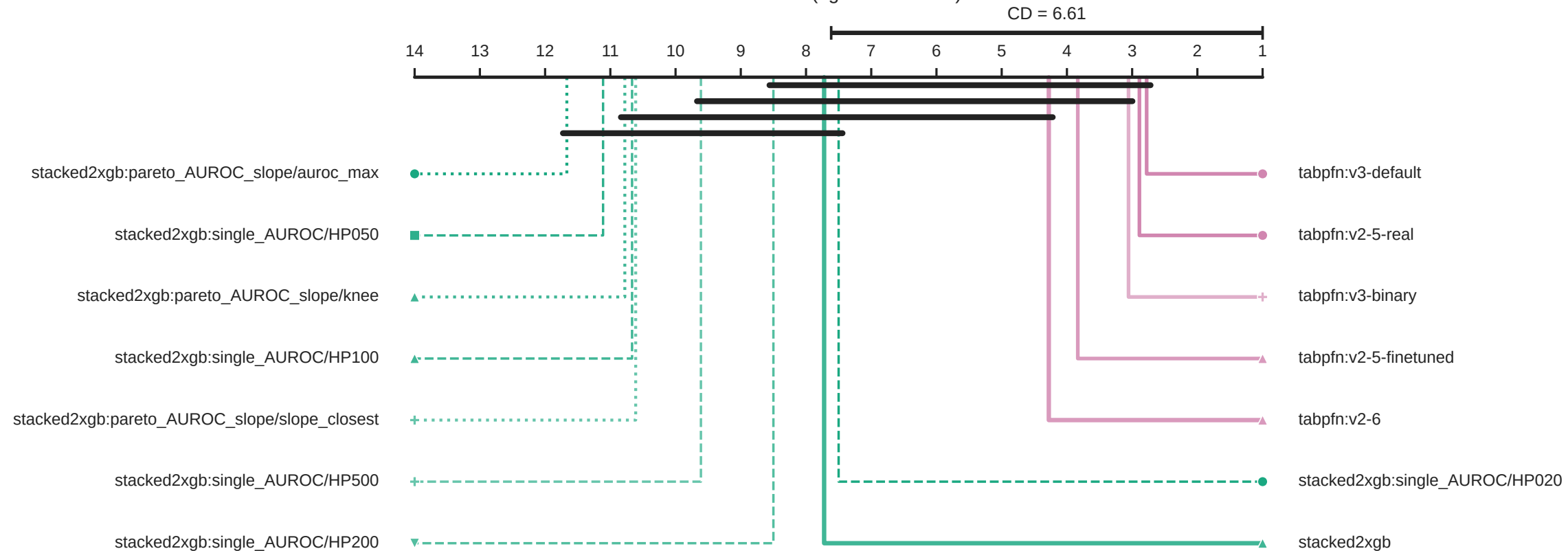
Critical Difference - headache AUROC (Park 2016 SHD, n=62) (Friedman p = 1.09e-11, n_cells = 9) Mean rank (rightmost = best)
