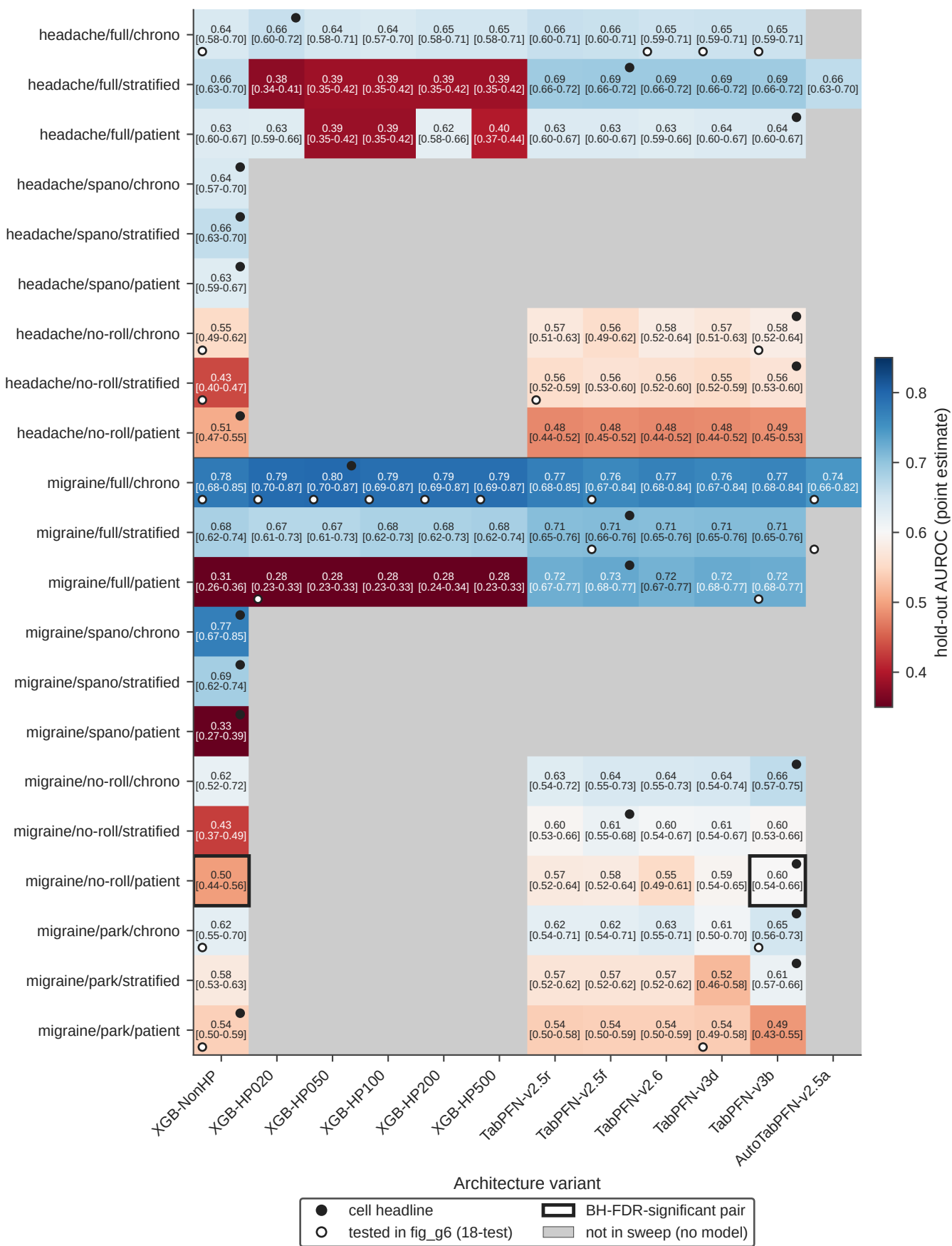
AUROC heatmap with main-text BH-FDR overlay (18-test targeted family)
