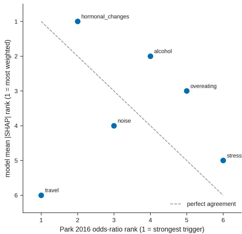
runner_up tabpfn - Spearman rho = -0.03
