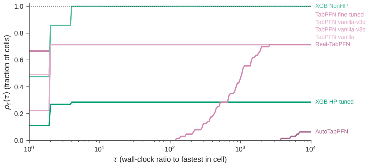
Performance profile (Dolan-More) of training wall-clock, 63 cells
