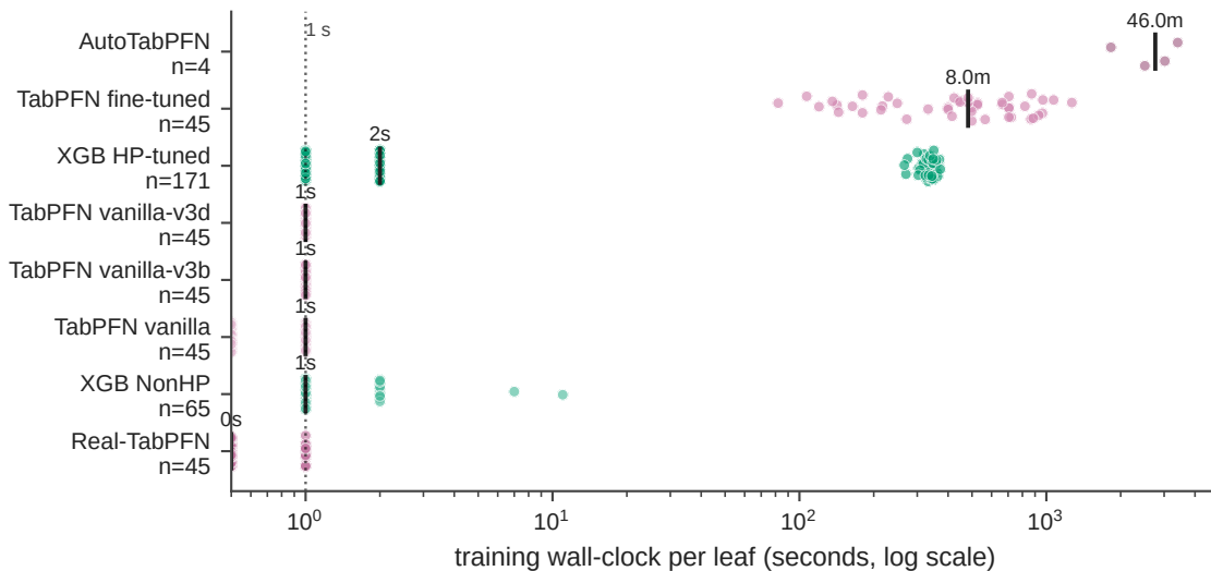
Training wall-clock per leaf, by architecture class
