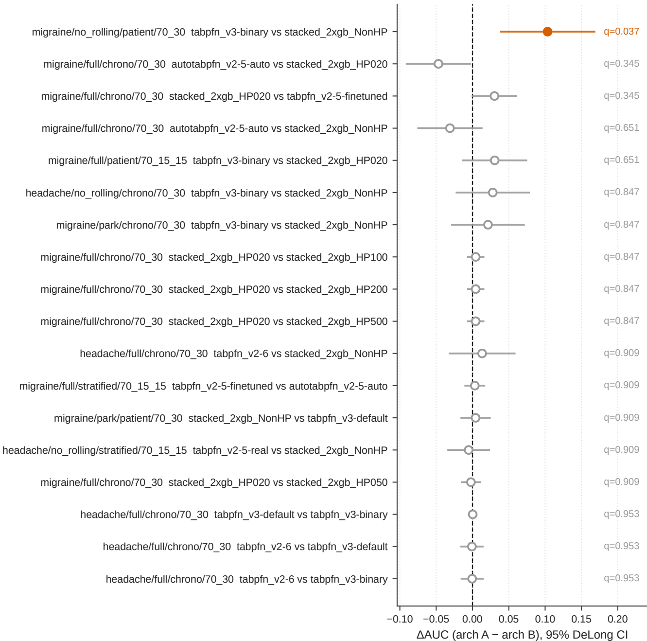
Paired DeLong + BH-FDR (q ≤ 0.05) across 18 cross-architecture tests; 1 significant after multiplicity correction
