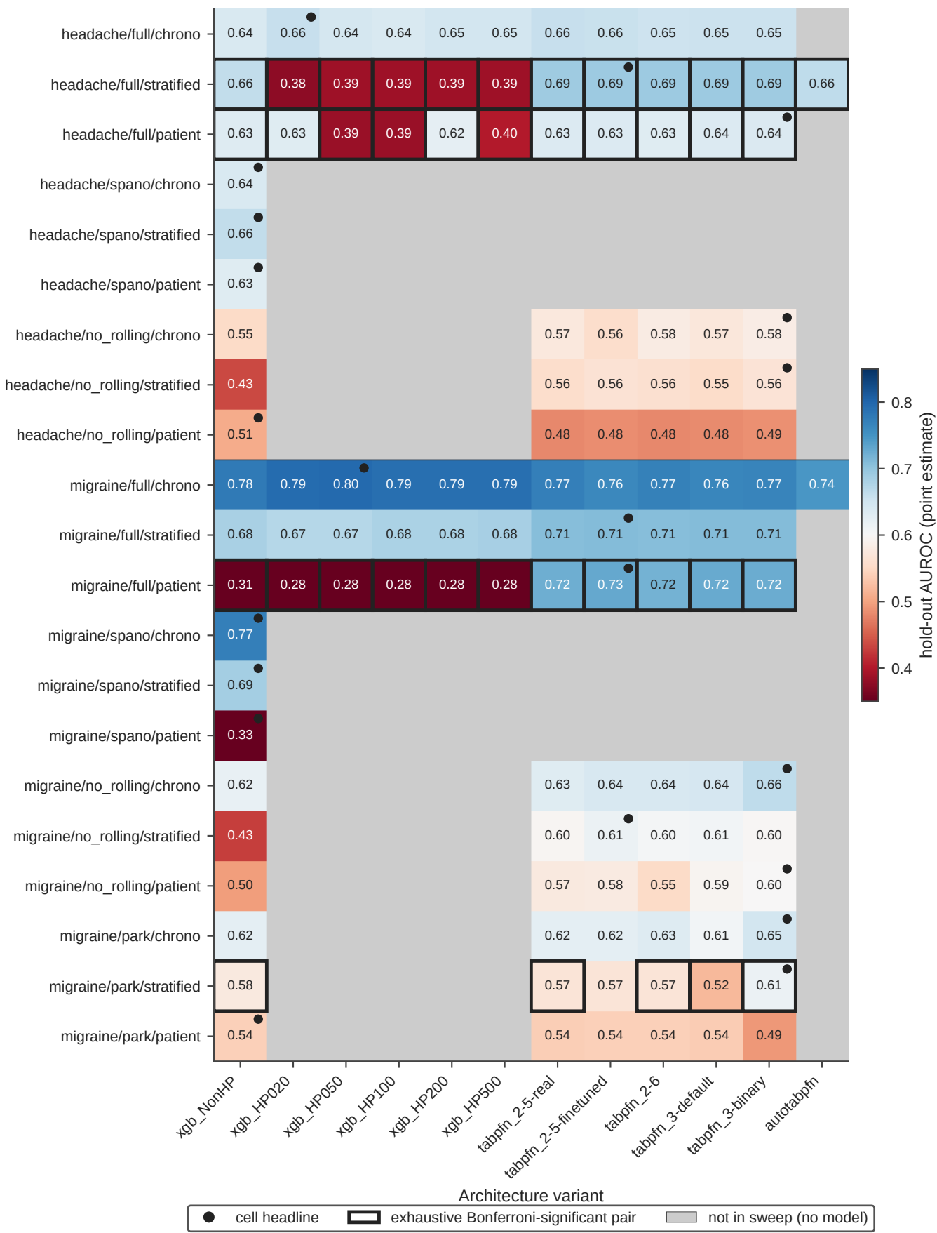
Supplementary AUROC heatmap at ratio 70_30 across the sweep
