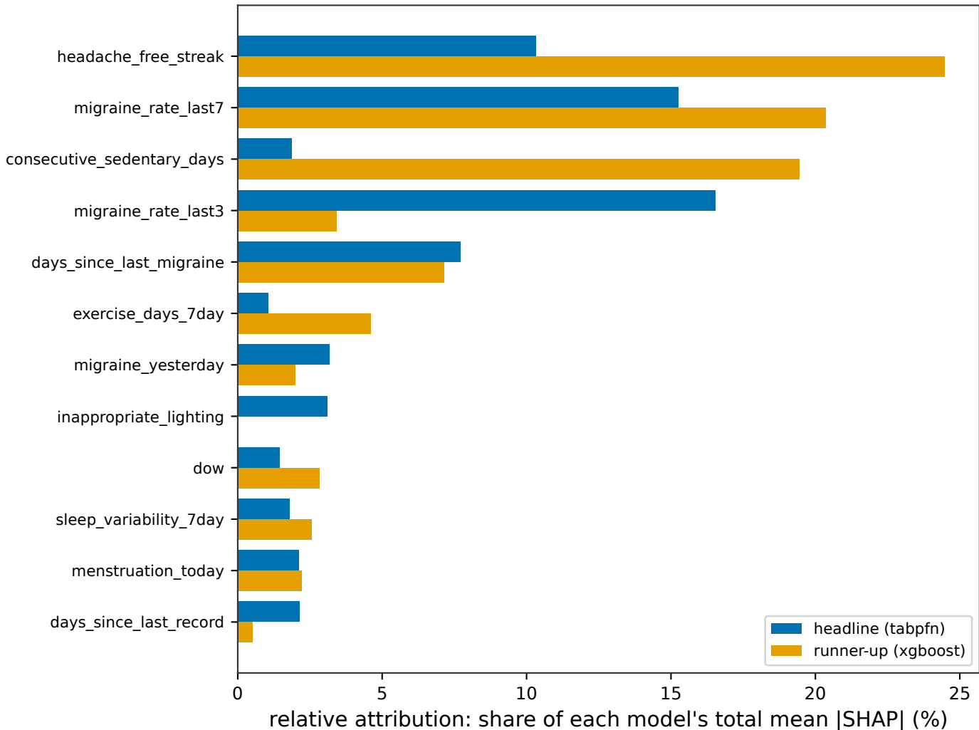
headache / full_features - chrono
