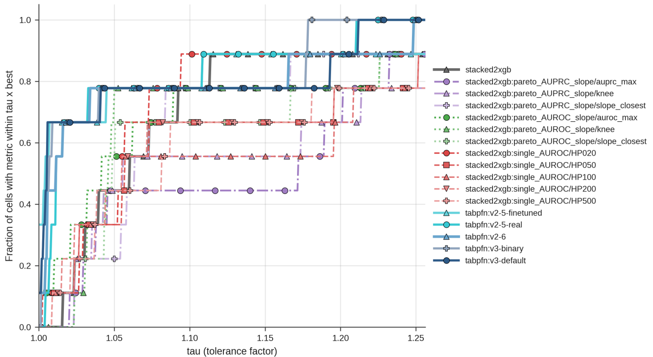
Performance profile (Dolan-More) - migraine AUROC (n_cells = 9)
