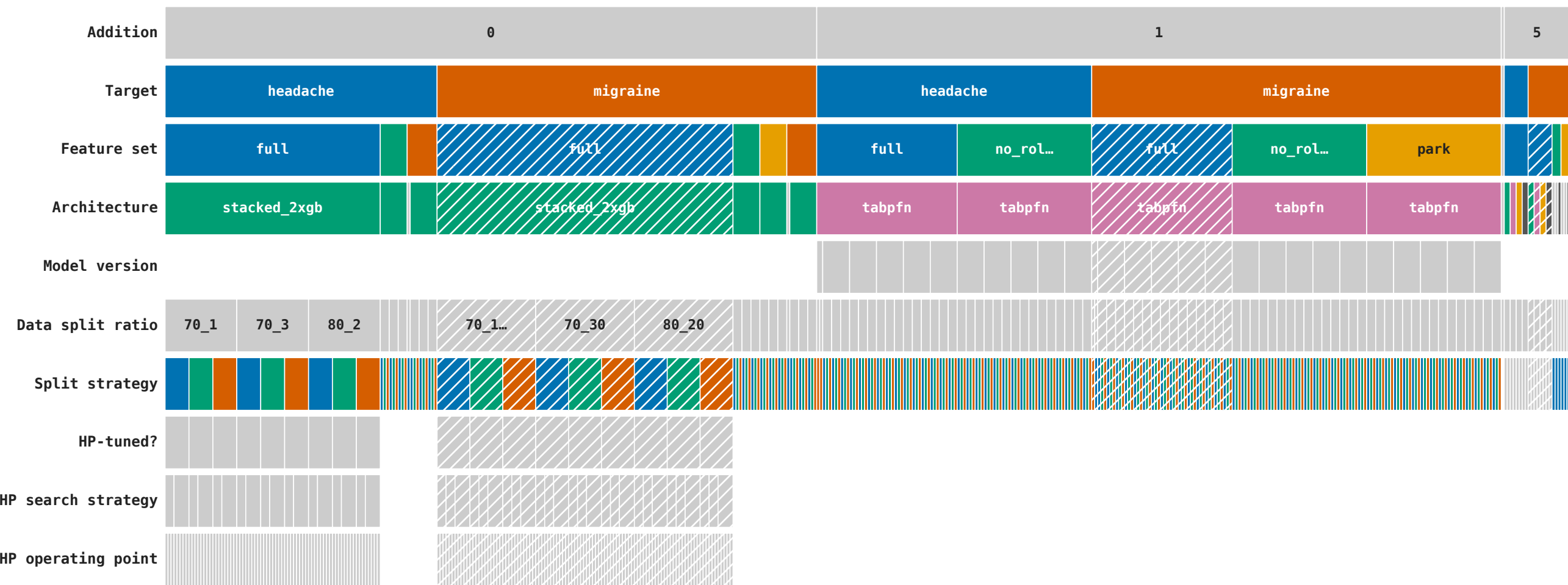
Discovered experiment leaves (470 total) - icicle plot
