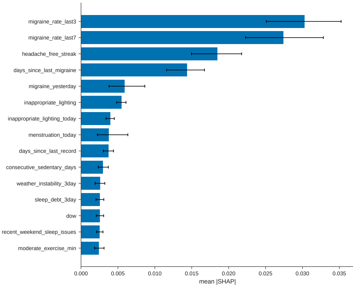
headache headline (TabPFN-v2.6 / full / chrono / 70-30) - feature attribution row-bootstrap 95% CI (n_boot=500, test rows n=40)
