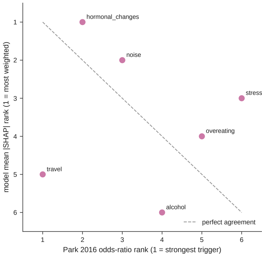
headline tabpfn - Spearman rho = +0.09, n = 6
