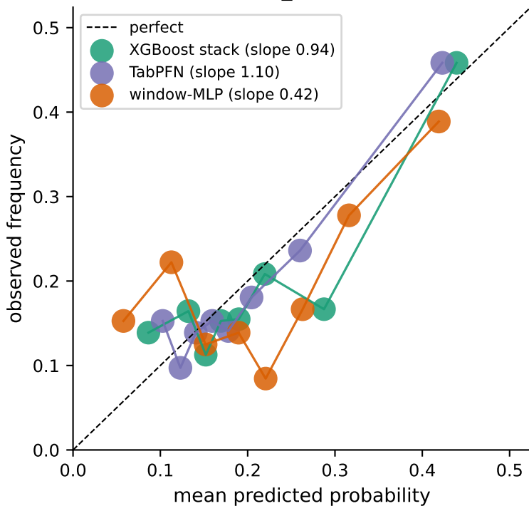
headache (full_features, chrono)
