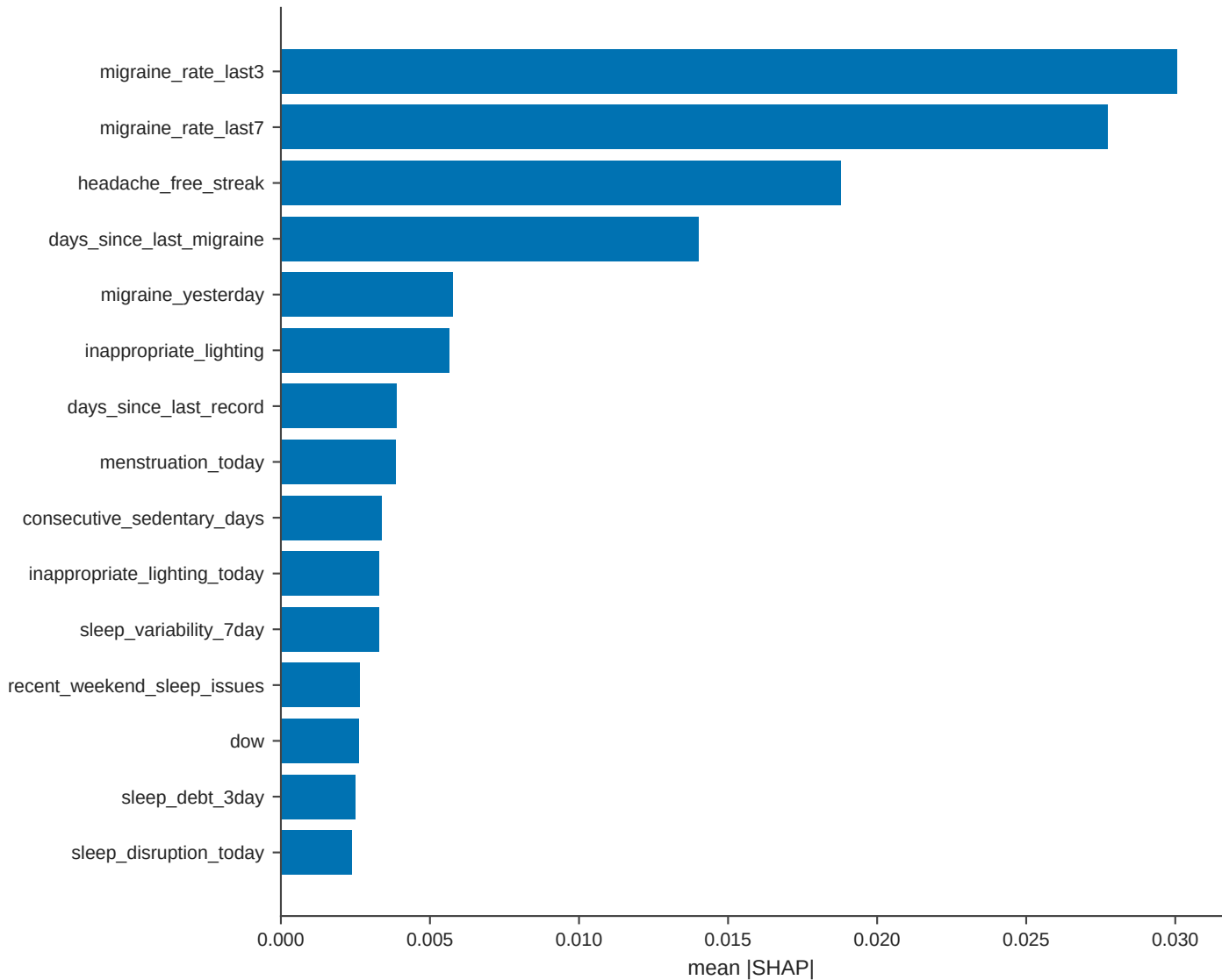
headache headline (tabpfn) - feature attribution
