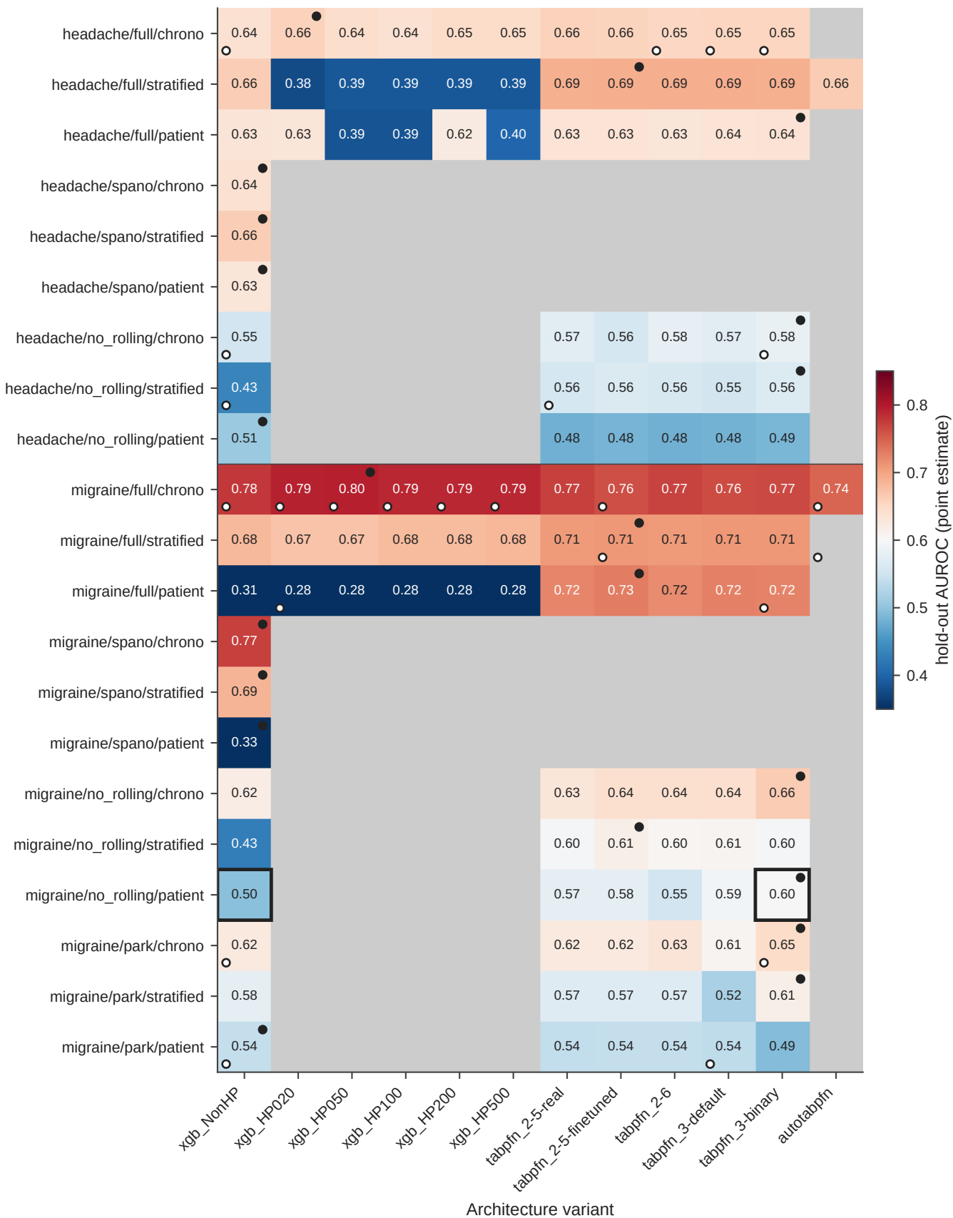
AUROC heatmap with main-text BH-FDR overlay (18-test targeted family) cell-headline •••; tested-in-G6 ○ ○ ○; thick edge = BH-FDR-significant pair
