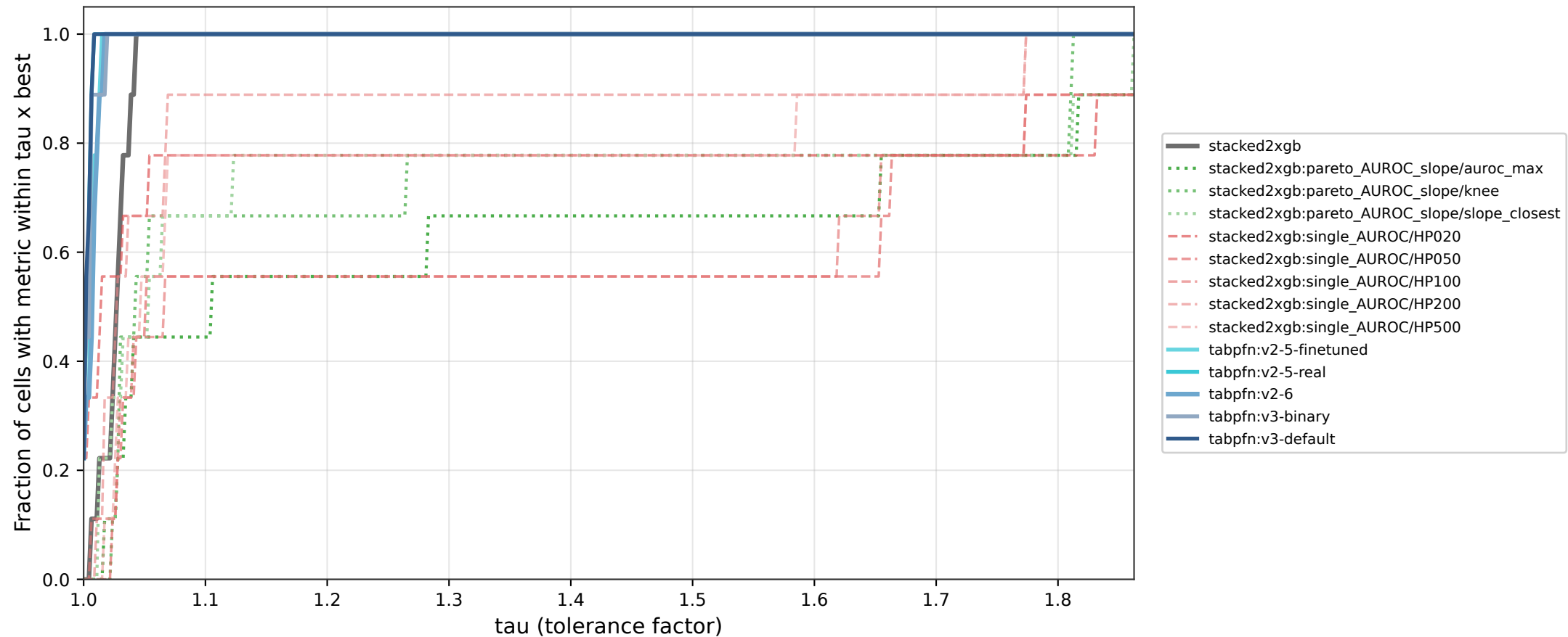
Performance profile (Dolan-More) - headache AUROC (n_cells = 9)
