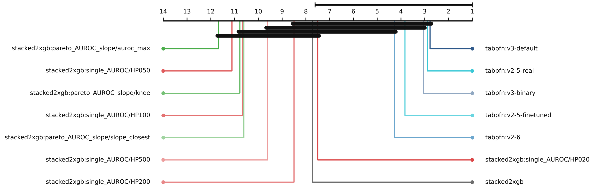
Critical Difference - headache AUROC (Friedman p = 1.09e-11, n cells = 9)
