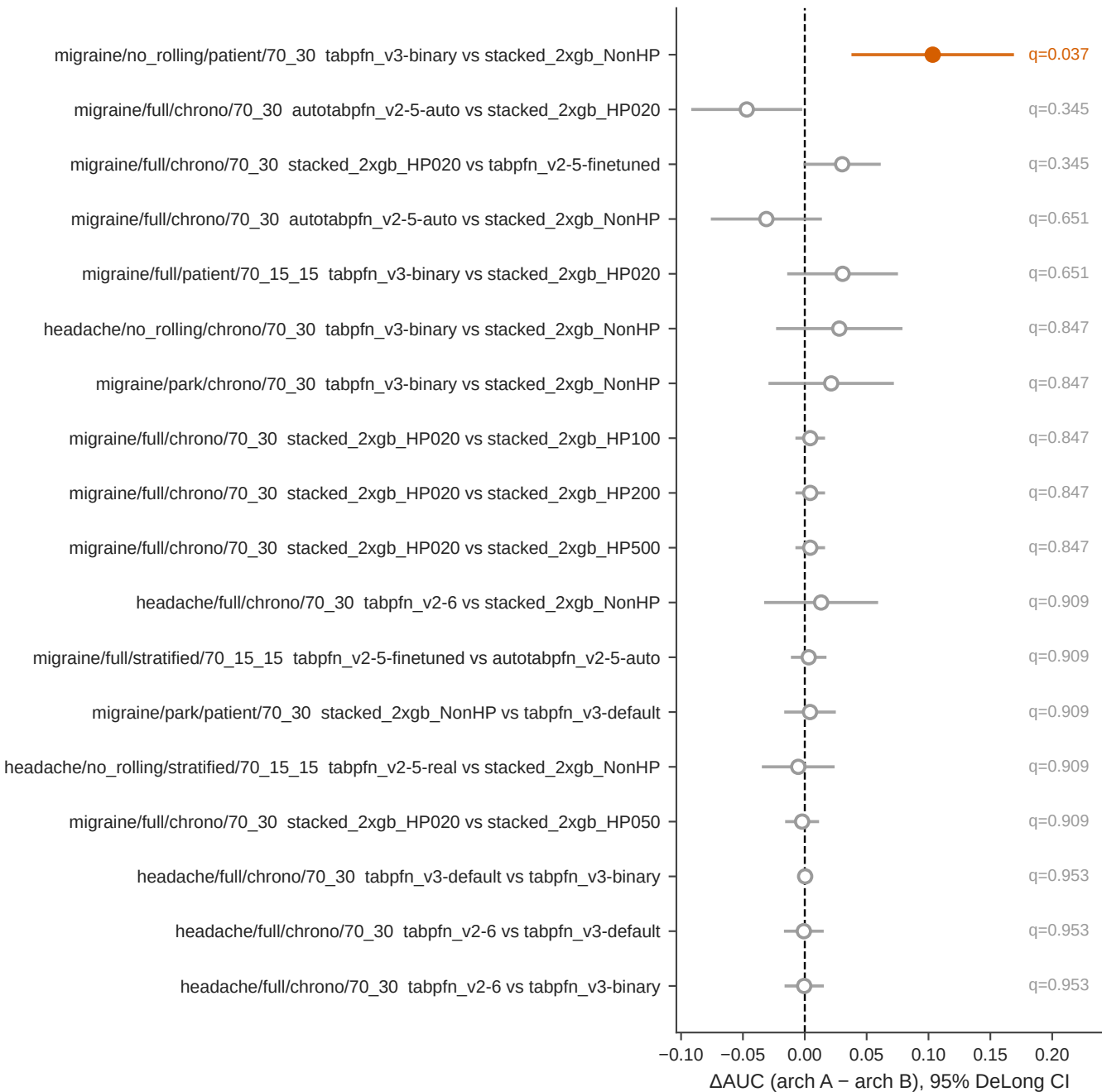
Paired DeLong + BH-FDR ( q \leq 0.05 ) across 18 cross-architecture tests; 1 significant after multiplicity correction
