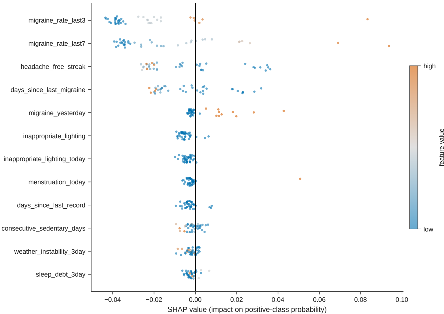
STAGE 1 / full_features / tabpfm (version_2-6) - per-row SHAP
