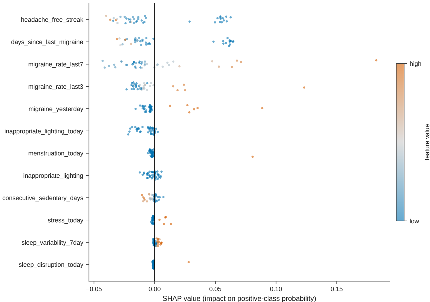
STAGE 1 / full_features / tabPFN (version_3-default) - per-row SHAP
