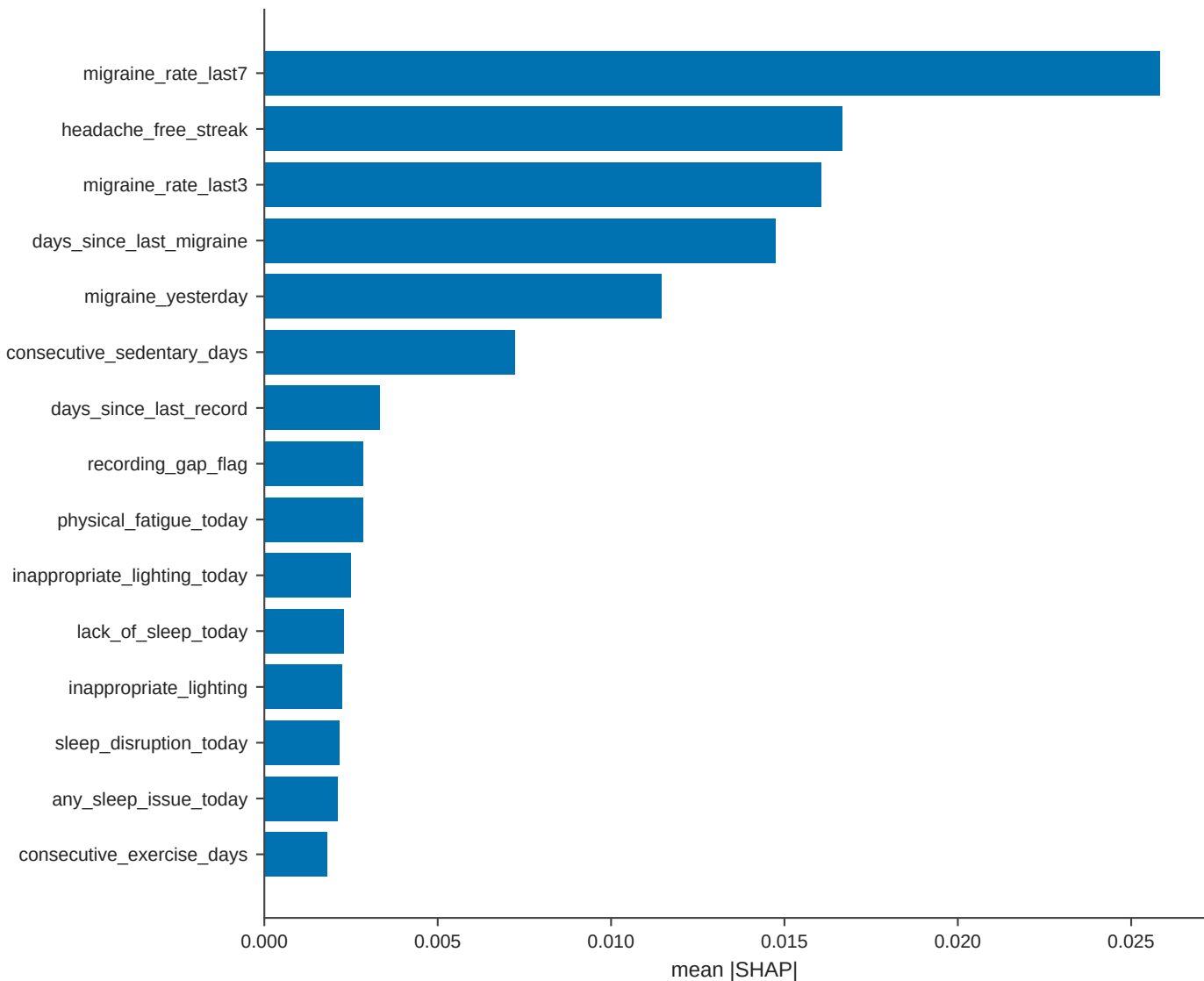
STAGE 1 / full_features / tabPFN (version_3-default) - feature attribution
