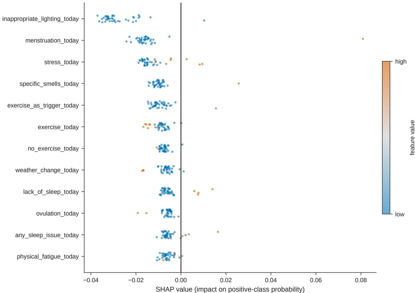
STAGE 1 / no_rolling_features / tabPFN (version_2-5-finetuned) - per-row SHAP
