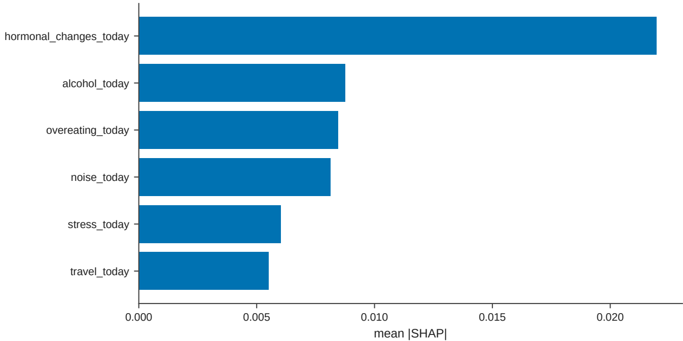
STAGE 1 / park_features / tabpfn (version_3-default) - feature attribution
