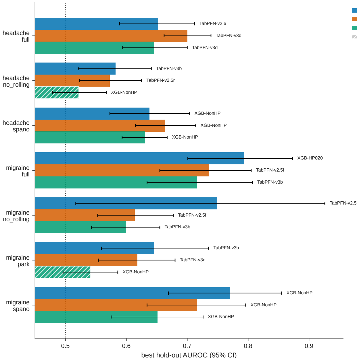
Discrimination by split type, per cell (headline model)
