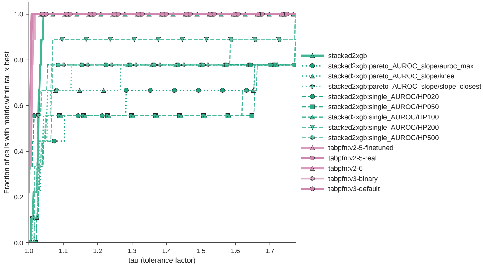
Performance profile (Dolan-More) - headache AUROC (n_cells = 9) · Park 2016 SHD (n=62)
