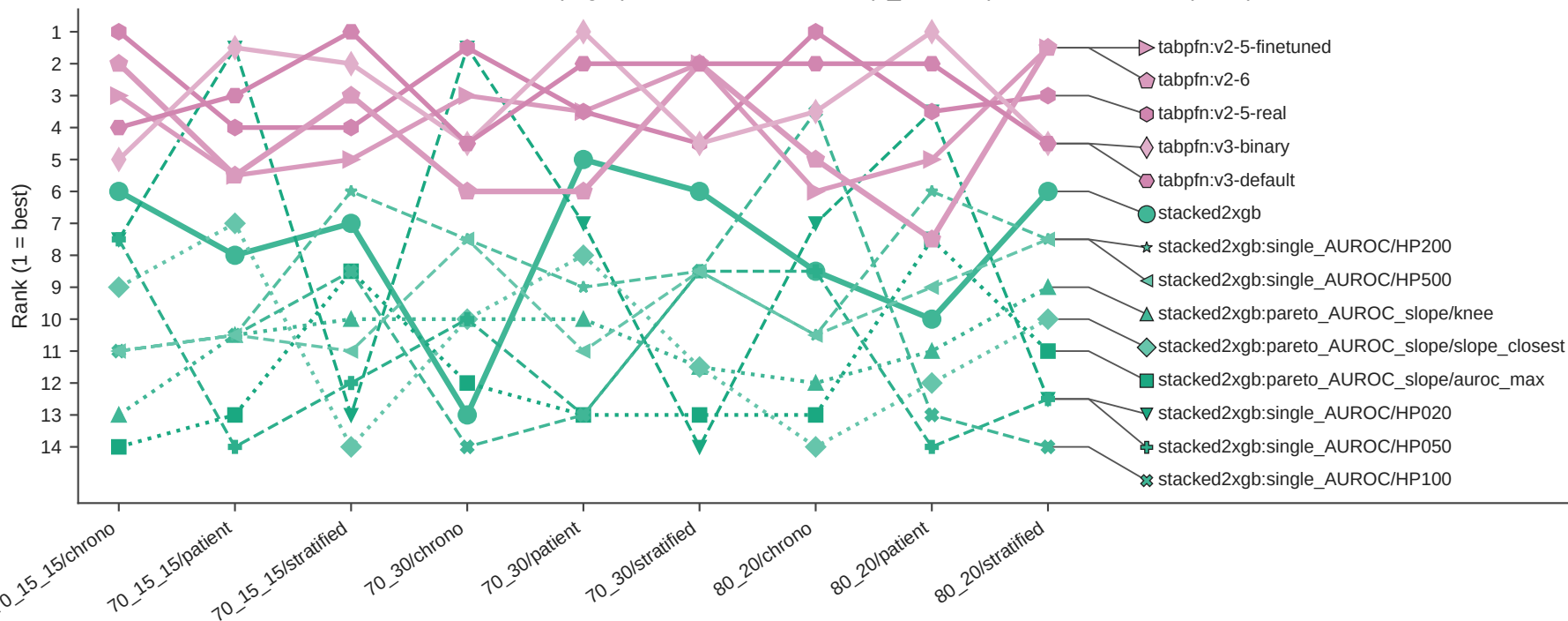
Rank slopegraph - headache AUROC (n_cells = 9) · Park 2016 SHD (n=62)
