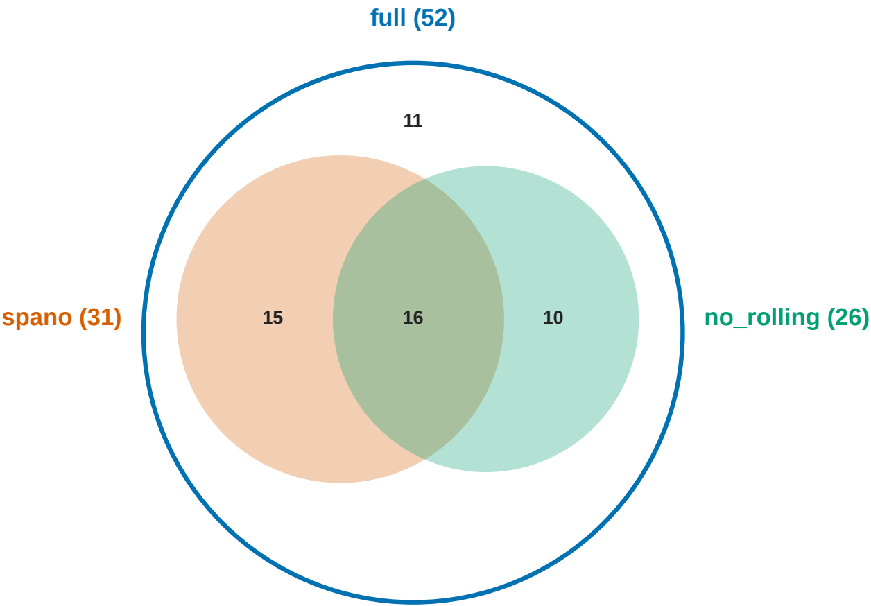
Feature-set structure - nested Euler (schematic) · Park 2016 SHD (n=62)
