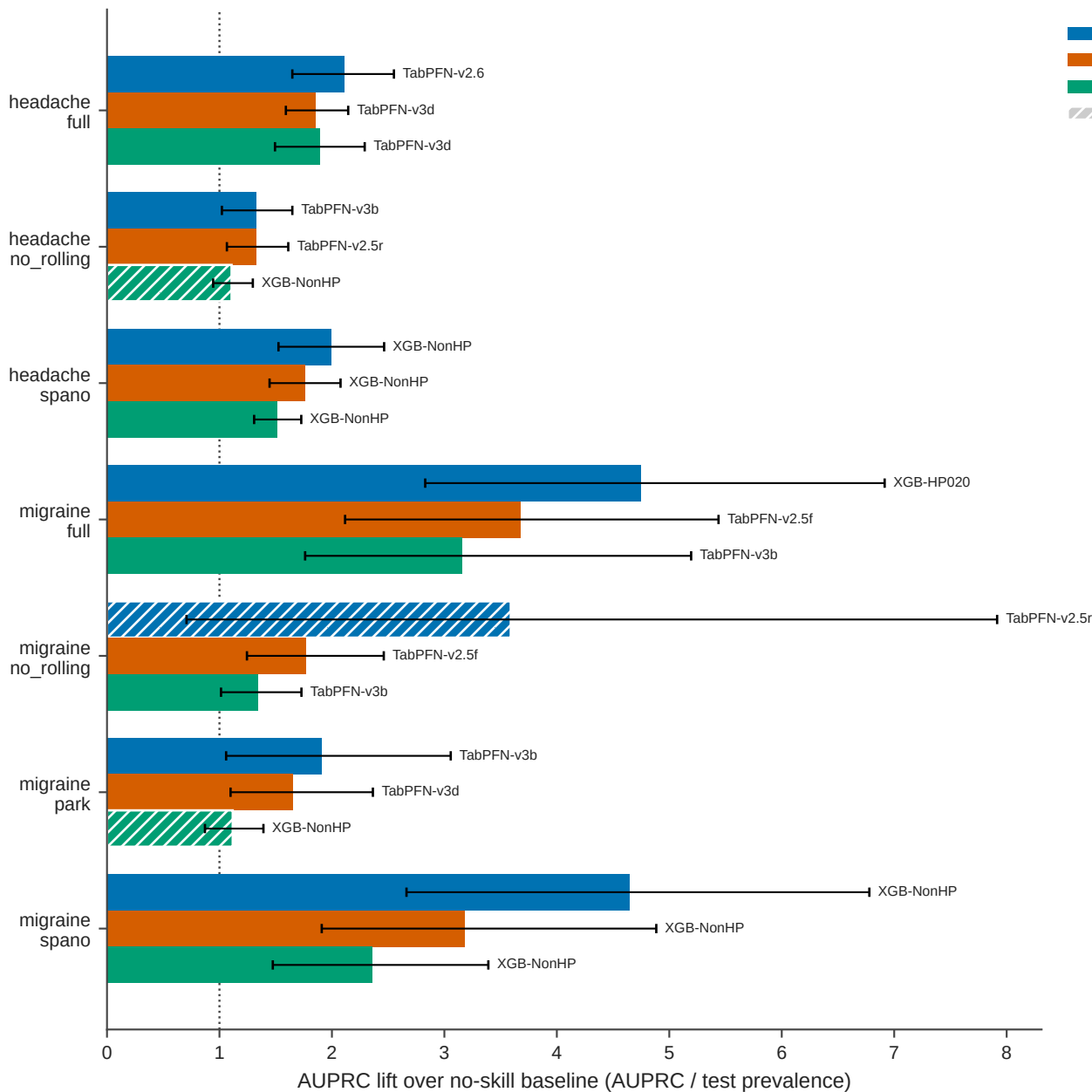
Precision-recall skill by split type, per cell (headline) · Park 2016 SHD (n=62)
