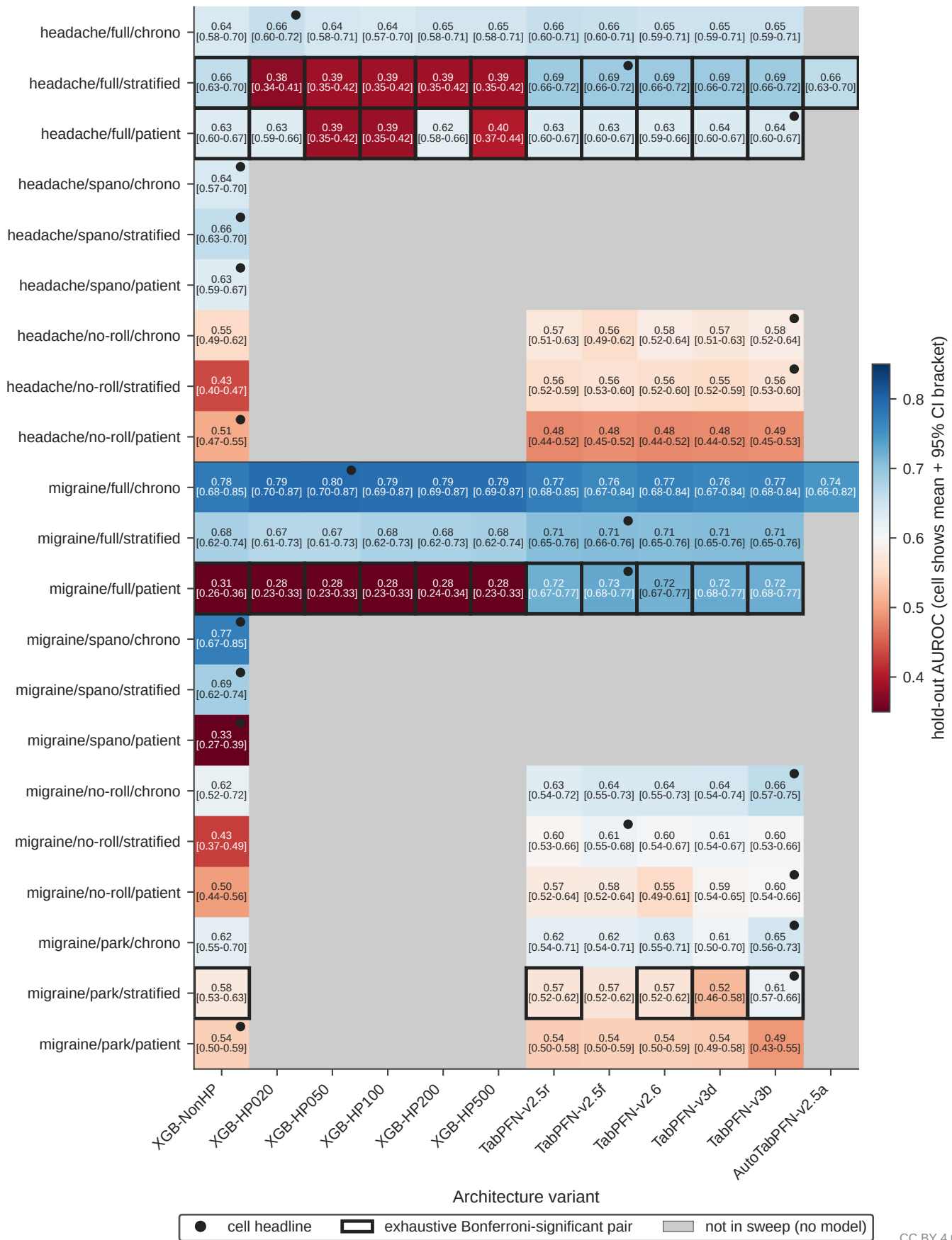
Supplementary AUROC heatmap at ratio 70_30 across the sweep · Park 2016 SHD (n=62)
