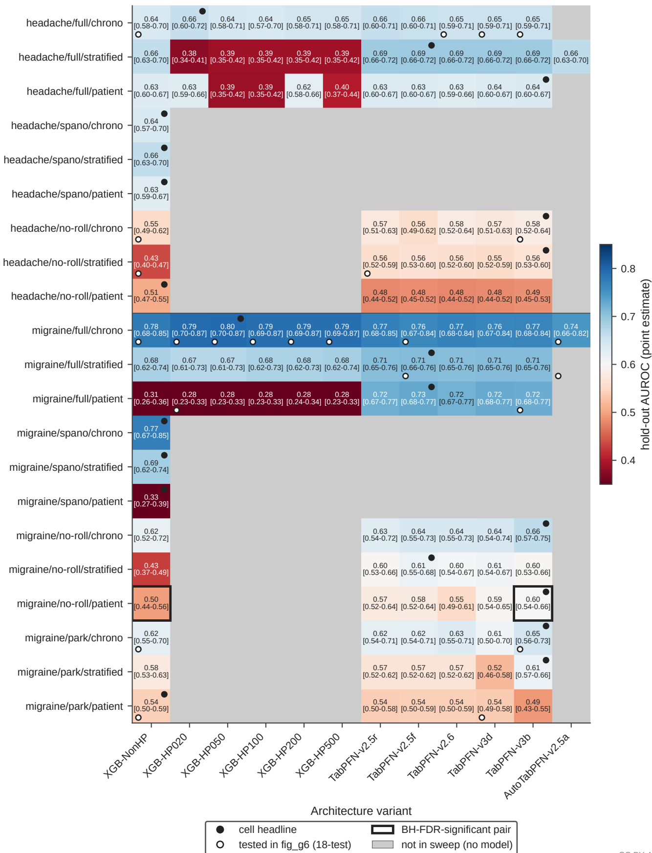
AUROC heatmap with main-text BH-FDR overlay (18-test targeted family) · Park 2016 SHD (n=62)
