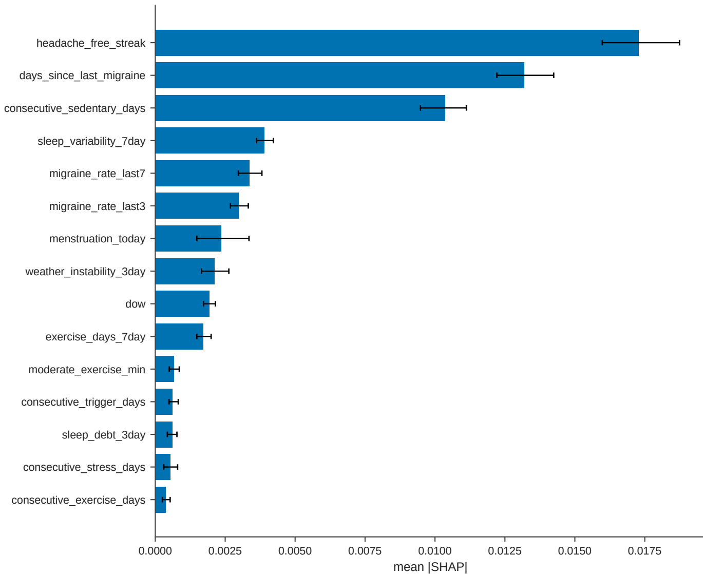
migraine headline (XGB-HP020 / full / chrono / 70-30) - feature attribution row-bootstrap 95% CI (n_boot=500, test rows n=400)
