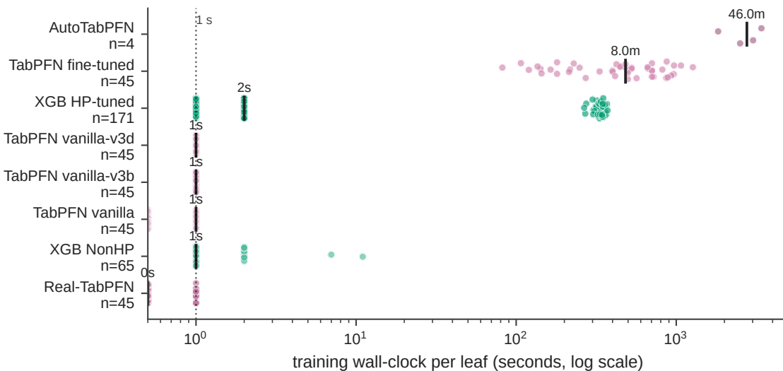
a Training wall-clock per leaf, by architecture class · Park 2016 SHD (n=62)
