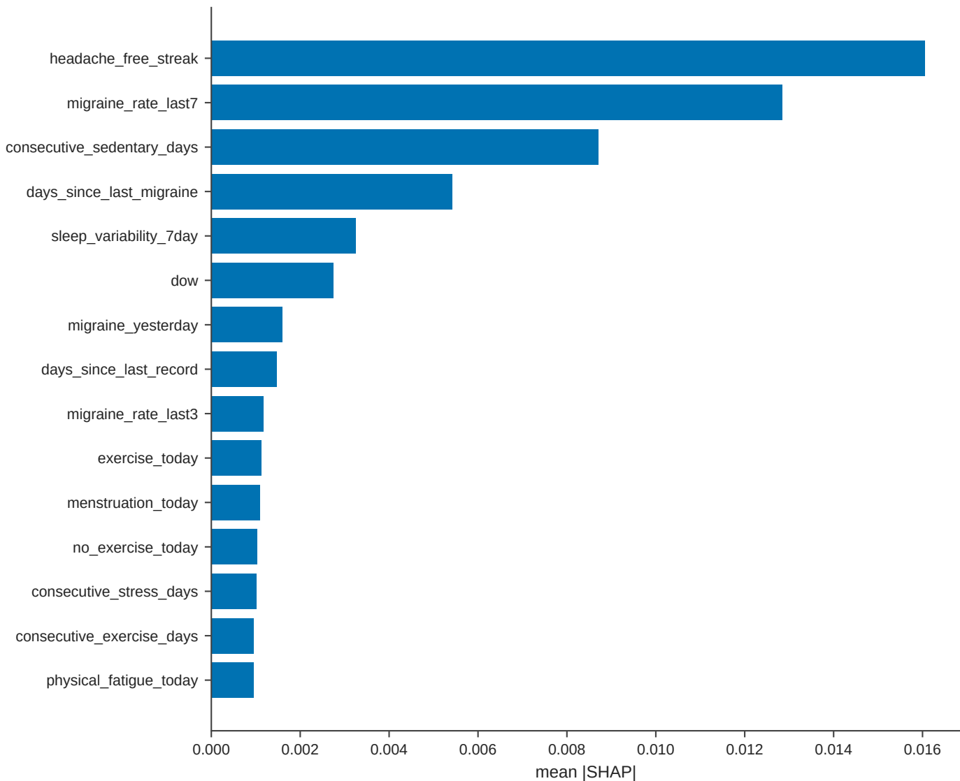
STAGE 0 / full_features / stacked_2xgb_meta_lr - feature attribution
