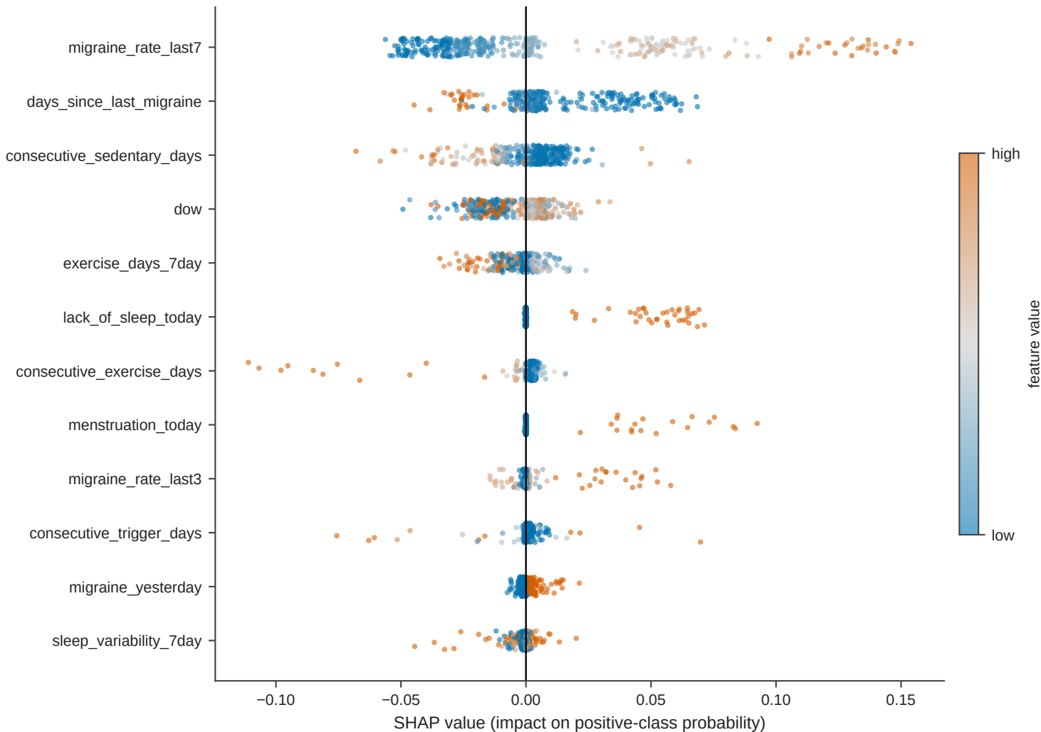
STAGE 0 / spano_features / stacked_2xgb_meta_lr - per-row SHAP
