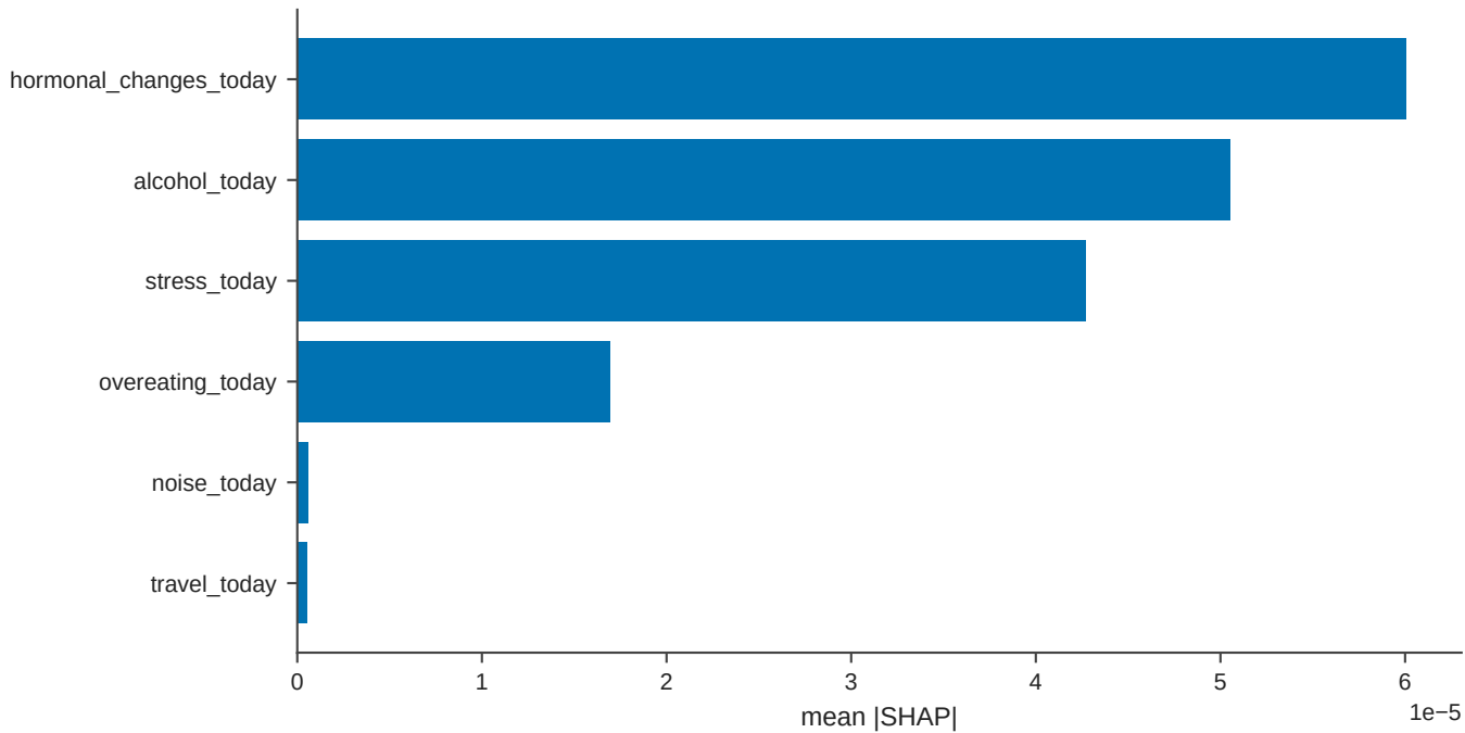
STAGE 0 / park_features / stacked_2xgb_meta_lr - feature attribution
