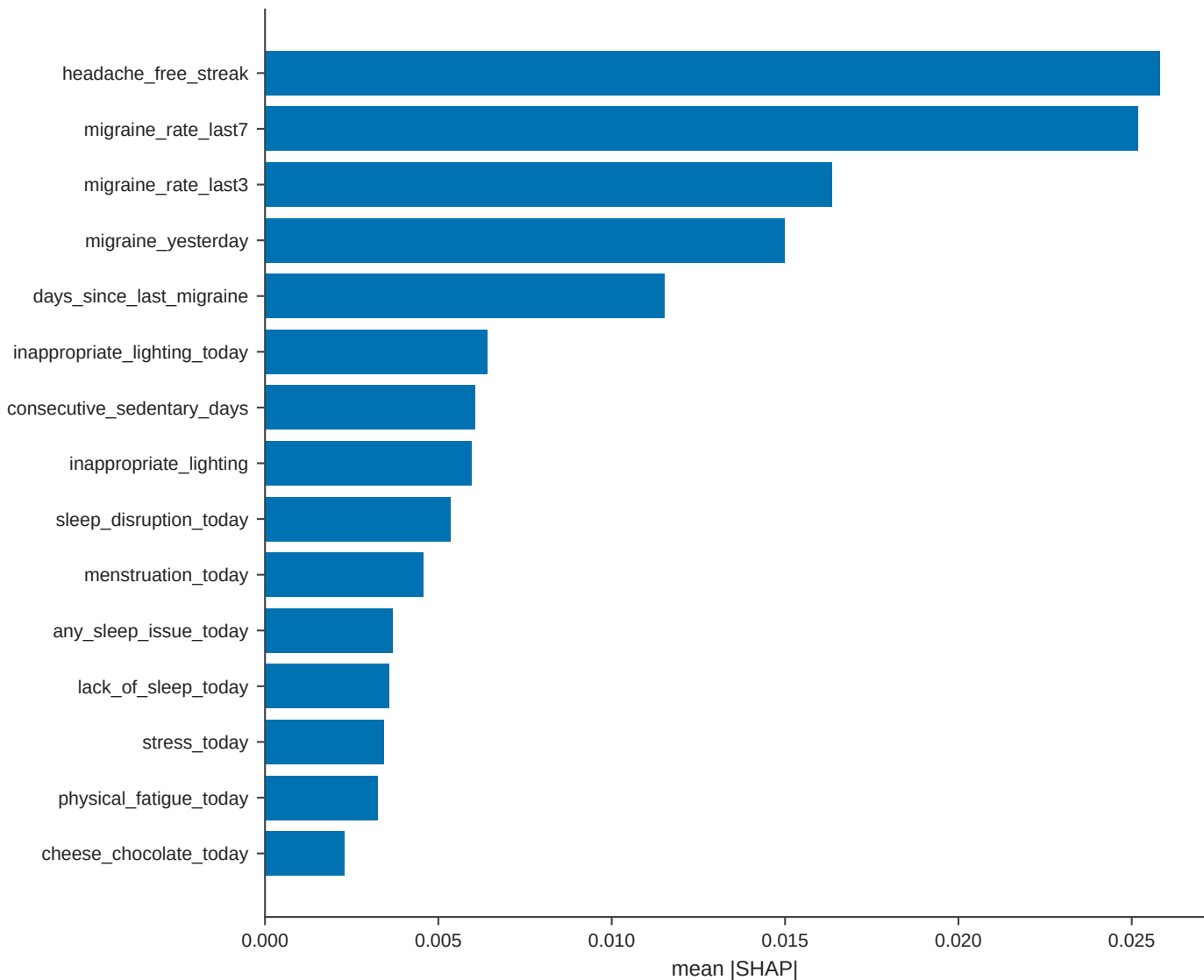
STAGE 1 / full_features / tabPFN (version_3-binary) - feature attribution
