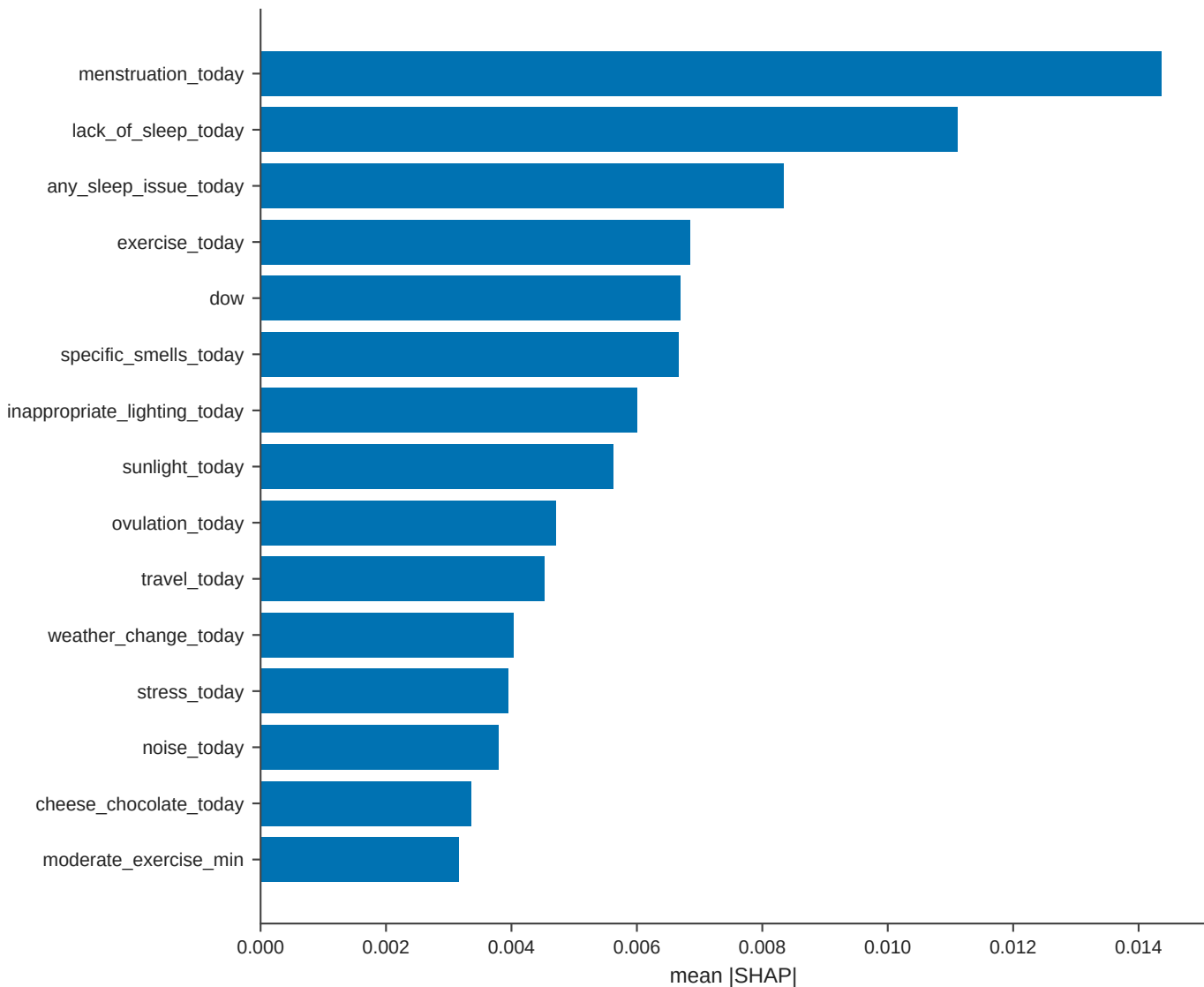
STAGE 1 / no_rolling_features / tabpfm (version_2-5-real) - feature attribution
