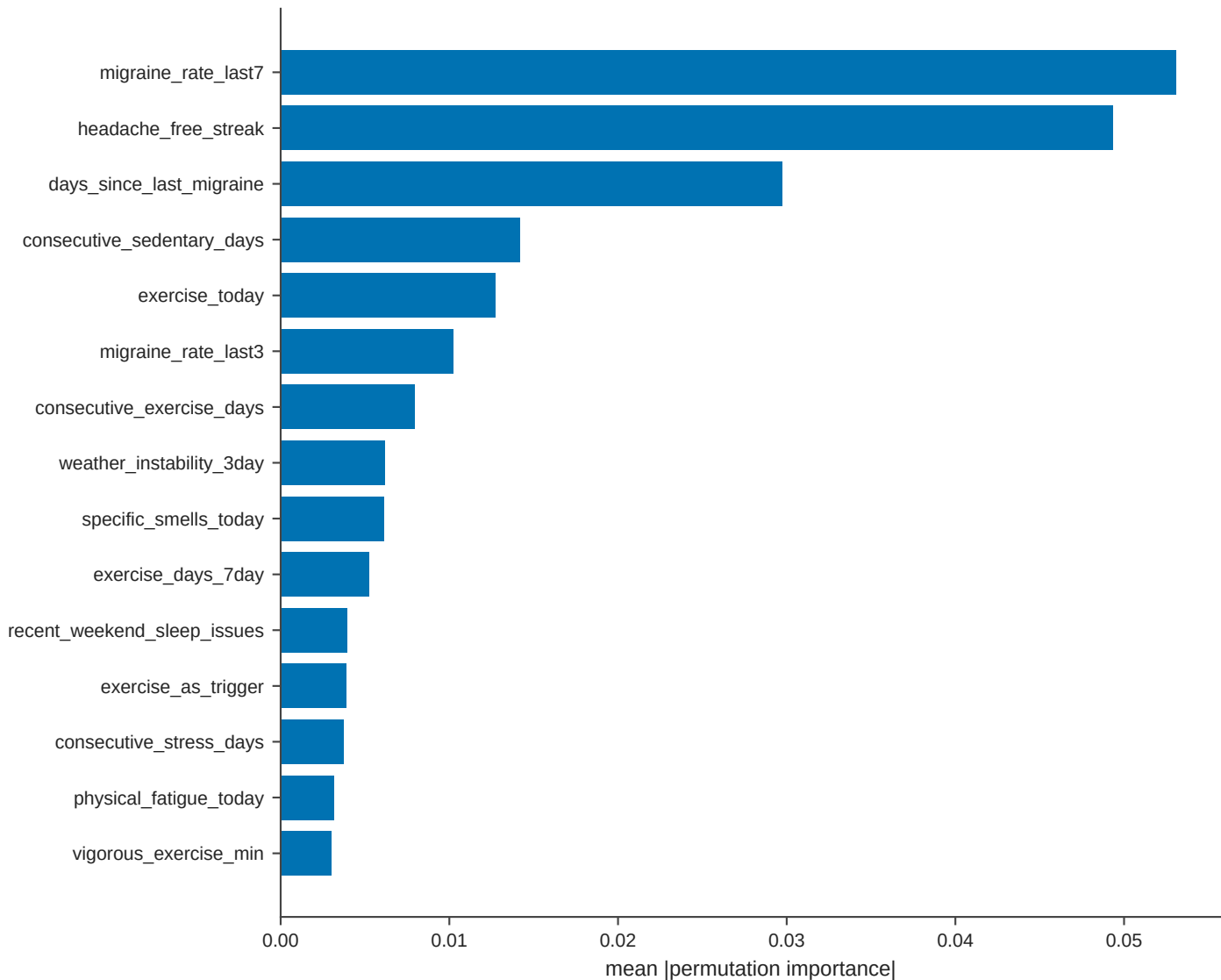
STAGE 1 / full_features / tabpfn (version_2-5-auto) - feature attribution
