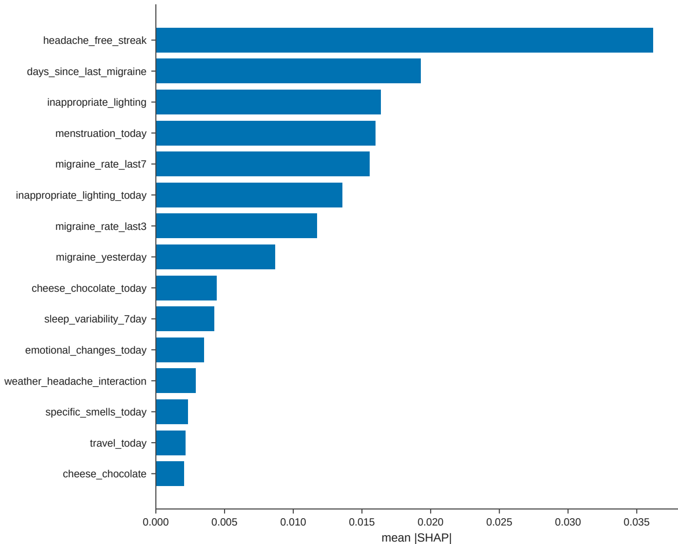
STAGE 1 / full_features / tabpfn (version_3-binary) - feature attribution
