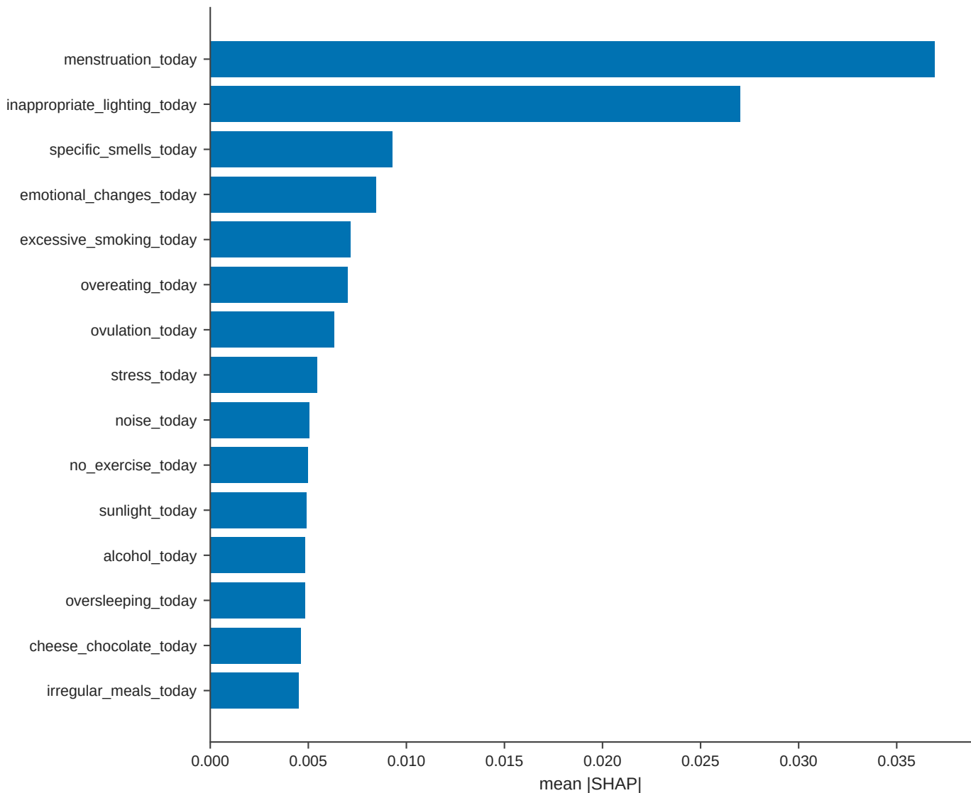
STAGE 1 / no_rolling_features / tabpfn (version_3-binary) - feature attribution
